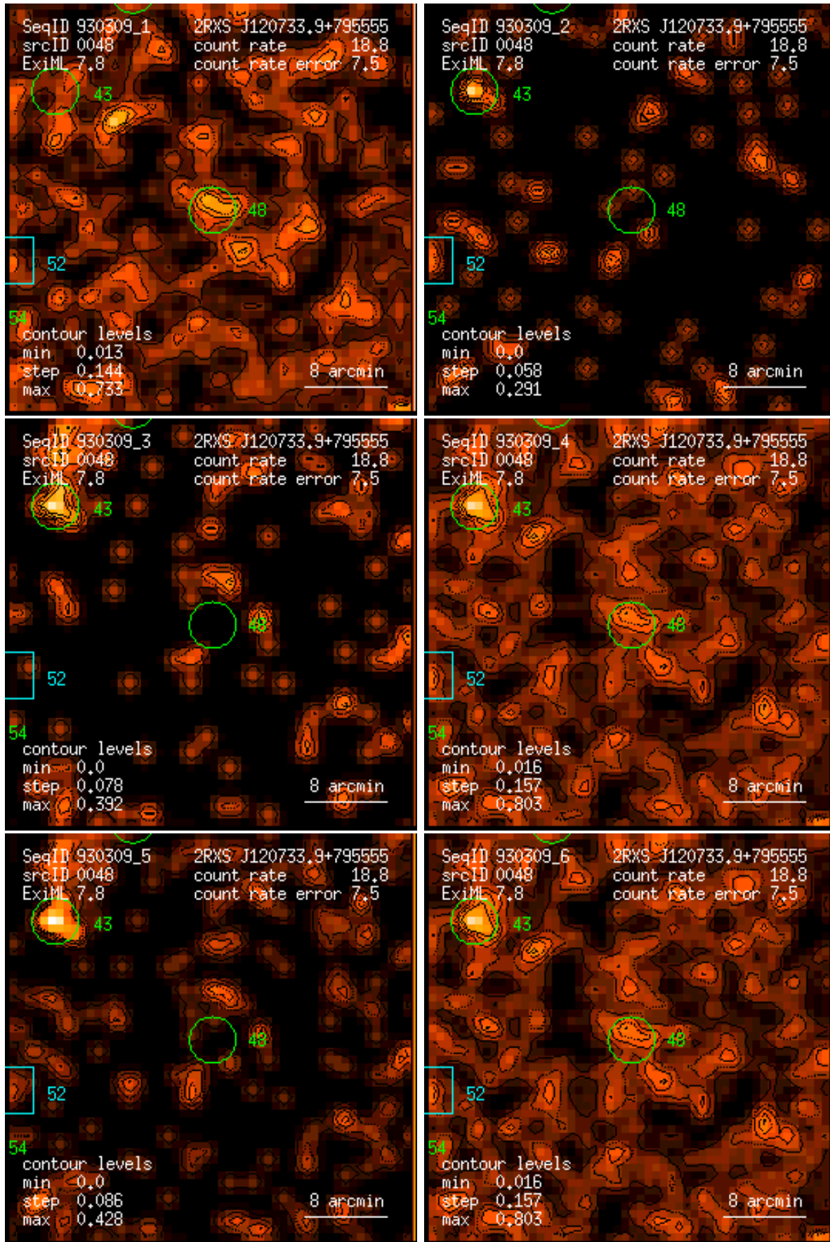
Figure 48: RASS 930309: detection 0048: band rate images, Gaussian filter: (1) PSPC channels 11 – 41, (2) 52 – 90, (3) 91 – 201, (4) 11 – 235, (5) 52 – 201, (6) 11 – 201. Broad band rates in counts/ks. Band rate contour levels in counts/ks/arcmin 2 .
