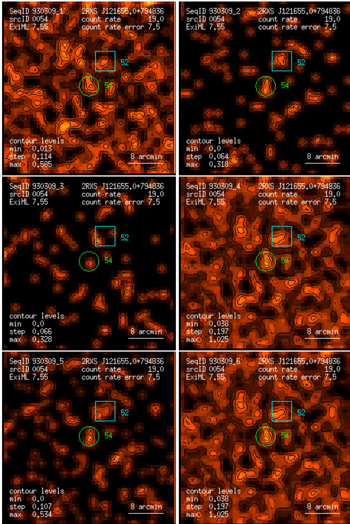
Figure 54: RASS 930309: detection 0054: band rate images, Gaussian filter: (1) PSPC channels 11 – 41, (2) 52 – 90, (3) 91 – 201, (4) 11 – 235, (5) 52 – 201, (6) 11 – 201. Broad band rates in counts/ks. Band rate contour levels in counts/ks/arcmin 2 .
