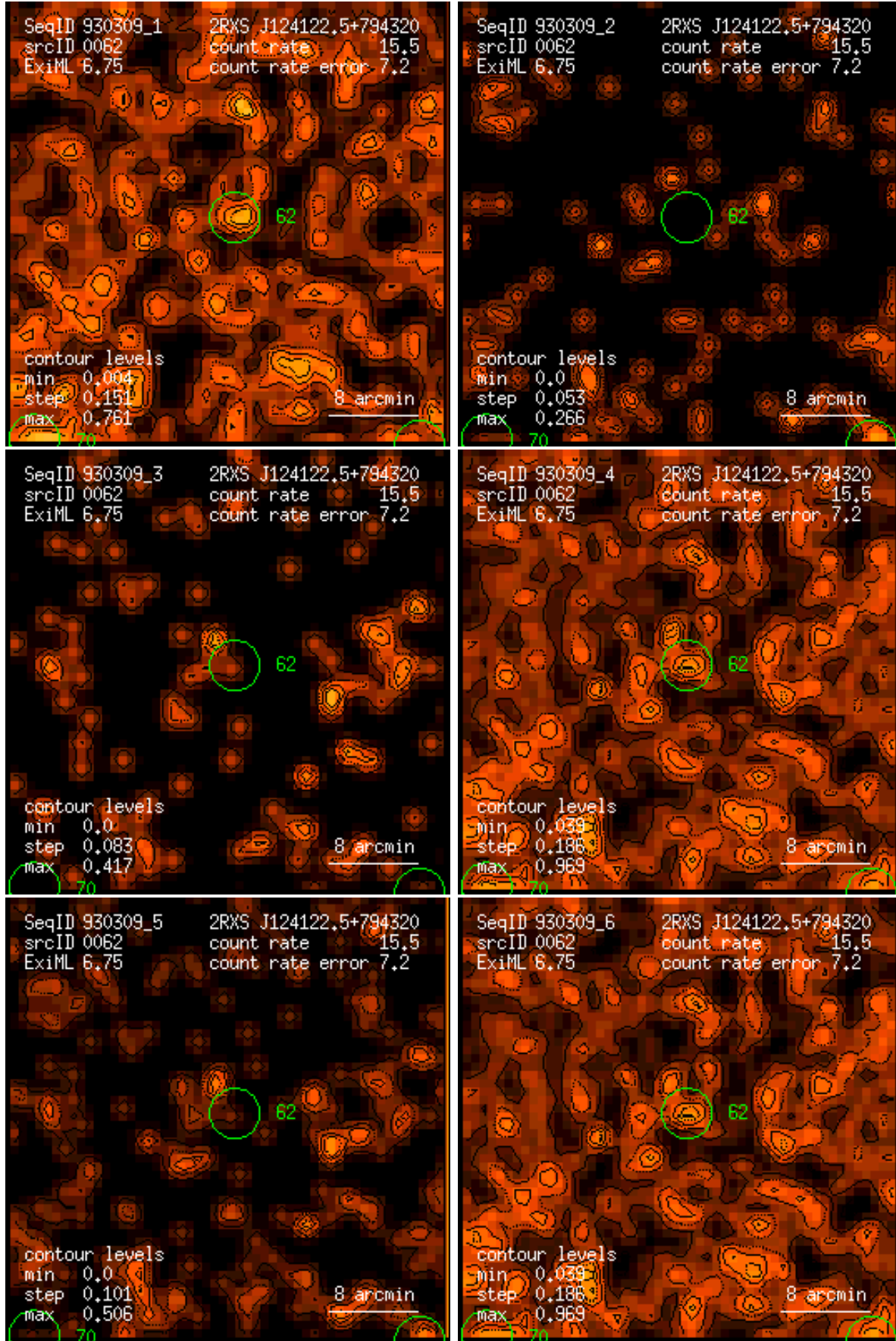
Figure 62: RASS 930309: detection 0062: band rate images, Gaussian filter: (1) PSPC channels 11 – 41, (2) 52 – 90, (3) 91 – 201, (4) 11 – 235, (5) 52 – 201, (6) 11 – 201. Broad band rates in counts/ks. Band rate contour levels in counts/ks/arcmin 2 .
