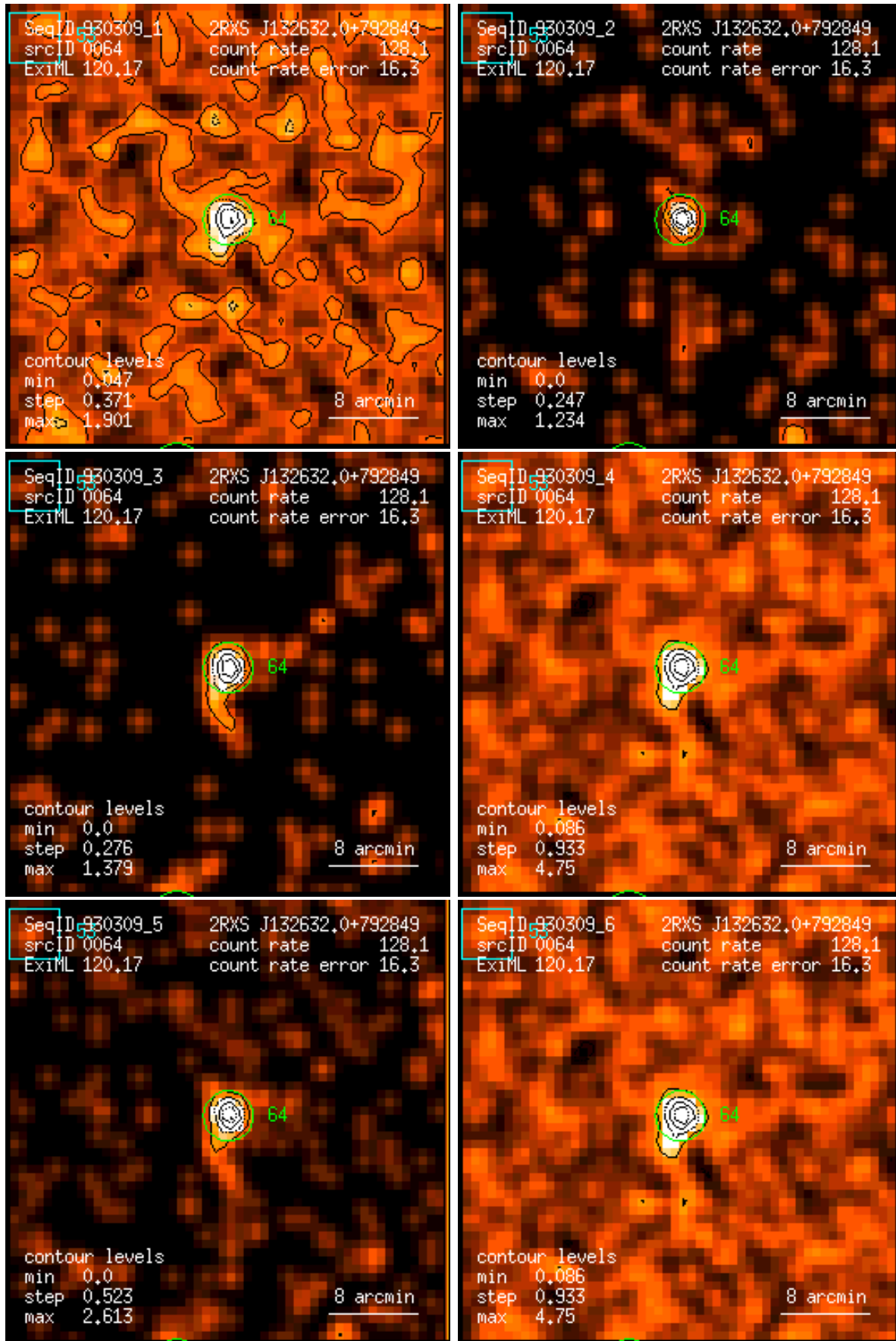
Figure 64: RASS 930309: detection 0064: band rate images, Gaussian filter: (1) PSPC channels 11 – 41, (2) 52 – 90, (3) 91 – 201, (4) 11 – 235, (5) 52 – 201, (6) 11 – 201. Broad band rates in counts/ks. Band rate contour levels in counts/ks/arcmin 2 .
