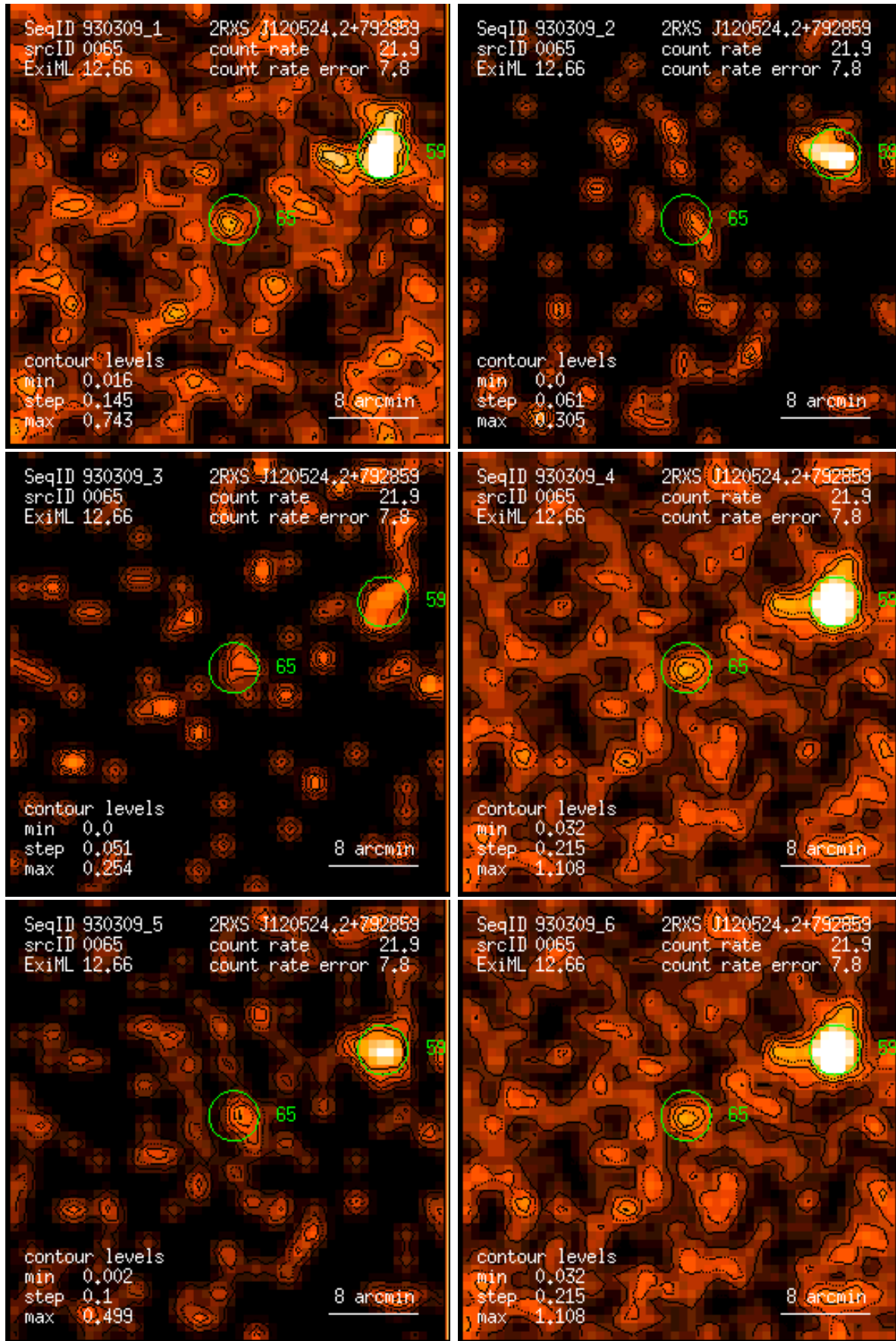
Figure 65: RASS 930309: detection 0065: band rate images, Gaussian filter: (1) PSPC channels 11 – 41, (2) 52 – 90, (3) 91 – 201, (4) 11 – 235, (5) 52 – 201, (6) 11 – 201. Broad band rates in counts/ks. Band rate contour levels in counts/ks/arcmin 2 .
