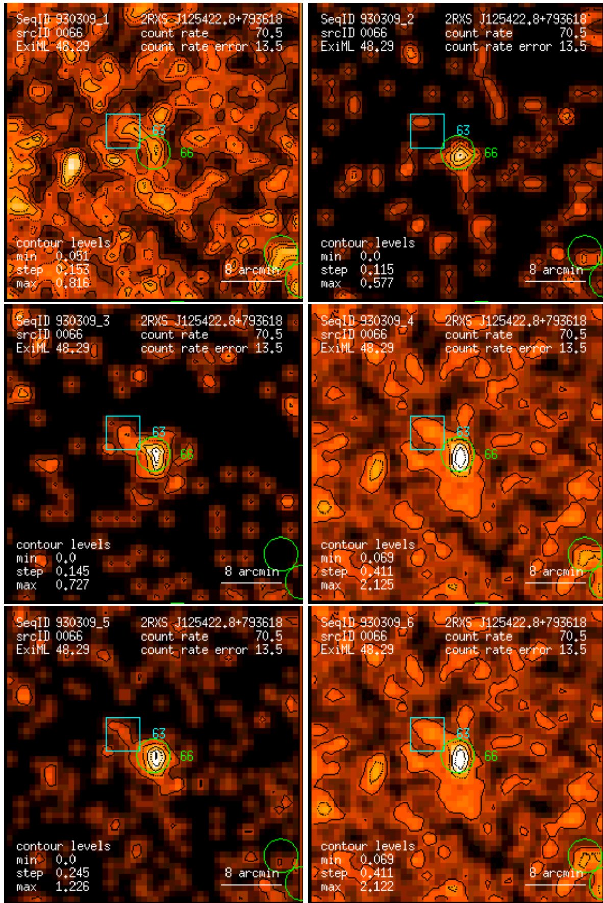
Figure 66: RASS 930309: detection 0066: band rate images, Gaussian filter: (1) PSPC channels 11 – 41, (2) 52 – 90, (3) 91 – 201, (4) 11 – 235, (5) 52 – 201, (6) 11 – 201. Broad band rates in counts/ks. Band rate contour levels in counts/ks/arcmin 2 .
