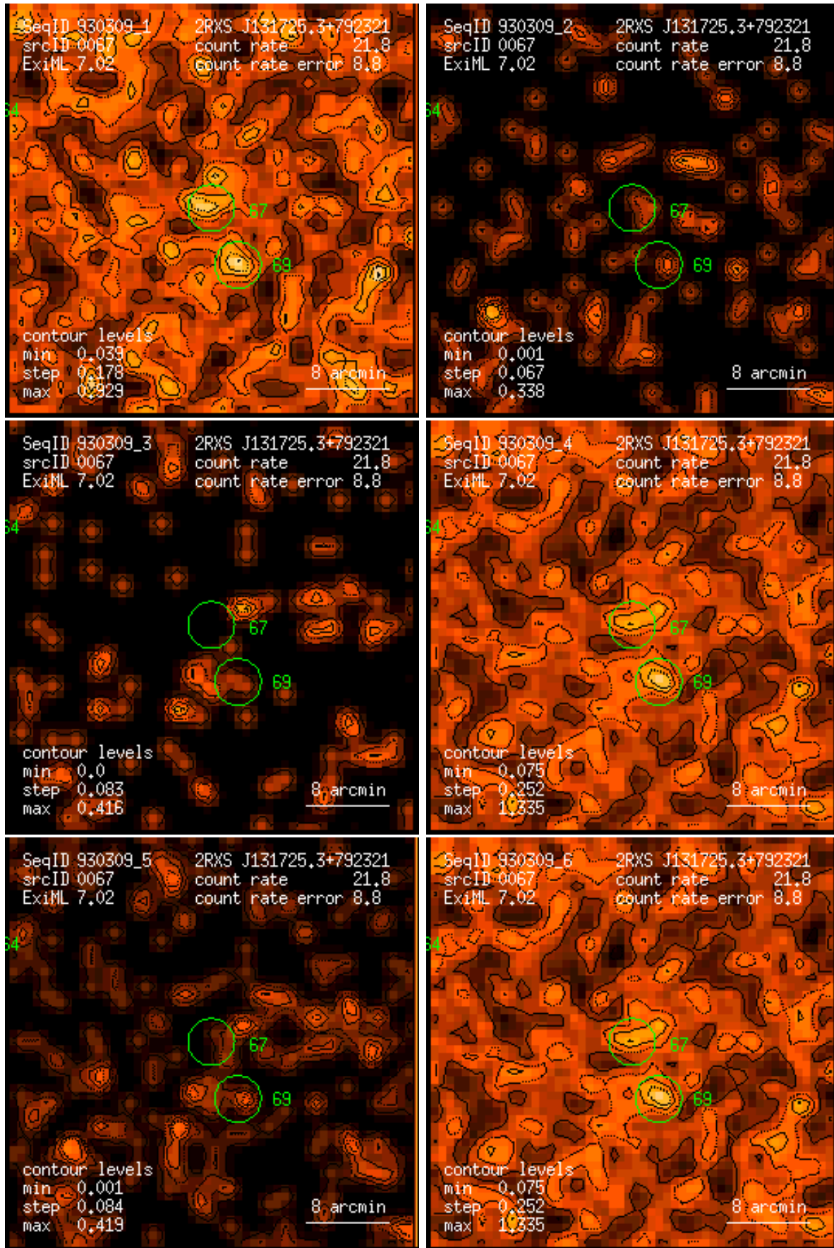
Figure 67: RASS 930309: detection 0067: band rate images, Gaussian filter: (1) PSPC channels 11 – 41, (2) 52 – 90, (3) 91 – 201, (4) 11 – 235, (5) 52 – 201, (6) 11 – 201. Broad band rates in counts/ks. Band rate contour levels in counts/ks/arcmin 2 .
