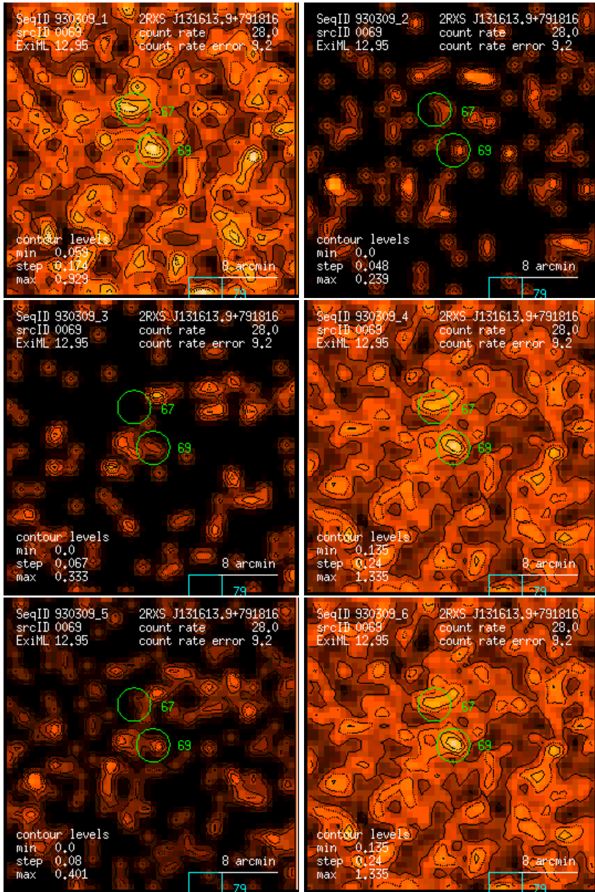
Figure 69: RASS 930309: detection 0069: band rate images, Gaussian filter: (1) PSPC channels 11 – 41, (2) 52 – 90, (3) 91 – 201, (4) 11 – 235, (5) 52 – 201, (6) 11 – 201. Broad band rates in counts/ks. Band rate contour levels in counts/ks/arcmin 2 .
