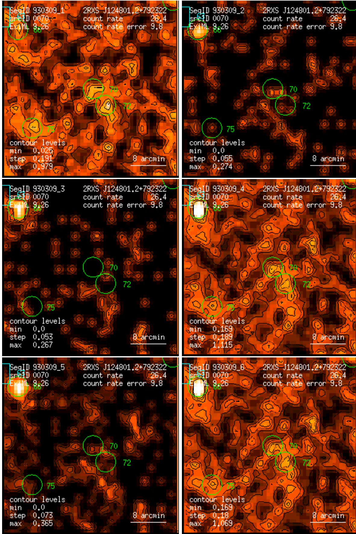
Figure 70: RASS 930309: detection 0070: band rate images, Gaussian filter: (1) PSPC channels 11 – 41, (2) 52 – 90, (3) 91 – 201, (4) 11 – 235, (5) 52 – 201, (6) 11 – 201. Broad band rates in counts/ks. Band rate contour levels in counts/ks/arcmin 2 .
