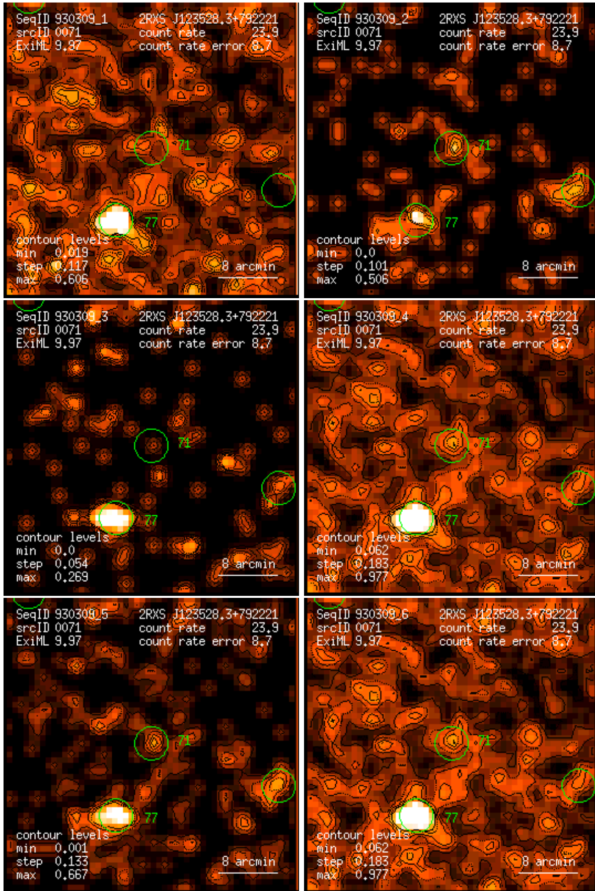
Figure 71: RASS 930309: detection 0071: band rate images, Gaussian filter: (1) PSPC channels 11 – 41, (2) 52 – 90, (3) 91 – 201, (4) 11 – 235, (5) 52 – 201, (6) 11 – 201. Broad band rates in counts/ks. Band rate contour levels in counts/ks/arcmin 2 .
