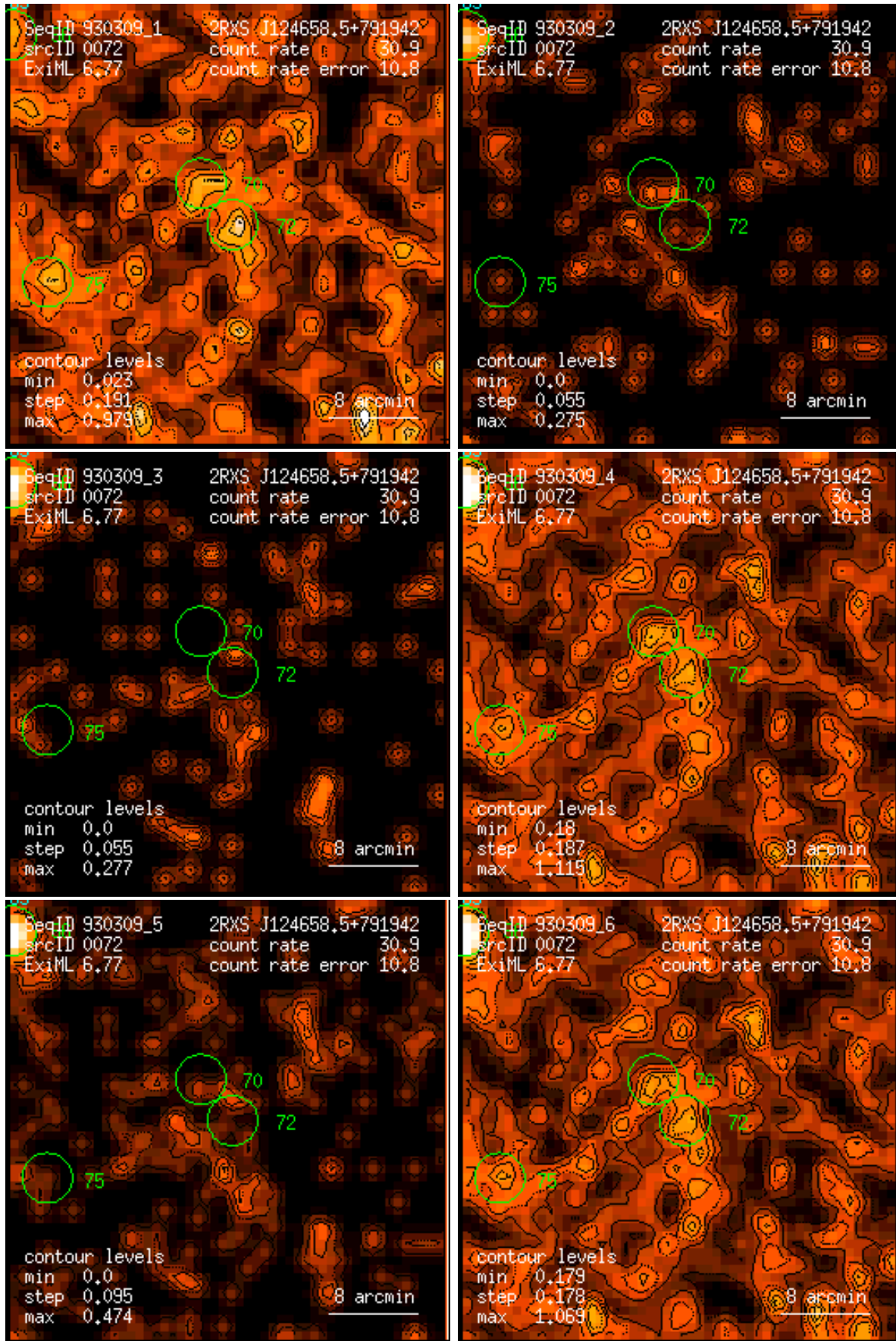
Figure 72: RASS 930309: detection 0072: band rate images, Gaussian filter: (1) PSPC channels 11 – 41, (2) 52 – 90, (3) 91 – 201, (4) 11 – 235, (5) 52 – 201, (6) 11 – 201. Broad band rates in counts/ks. Band rate contour levels in counts/ks/arcmin 2 .
