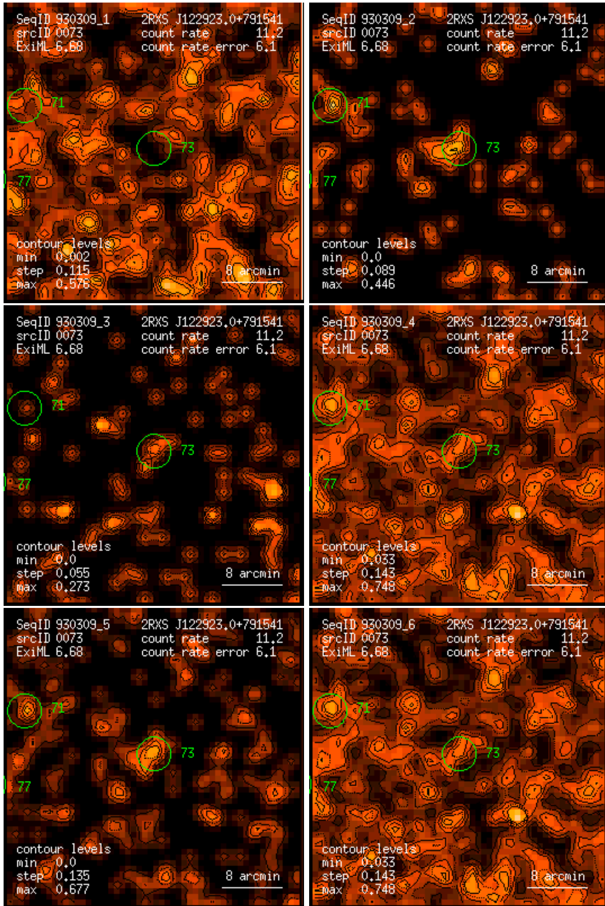
Figure 73: RASS 930309: detection 0073: band rate images, Gaussian filter: (1) PSPC channels 11 – 41, (2) 52 – 90, (3) 91 – 201, (4) 11 – 235, (5) 52 – 201, (6) 11 – 201. Broad band rates in counts/ks. Band rate contour levels in counts/ks/arcmin 2 .
