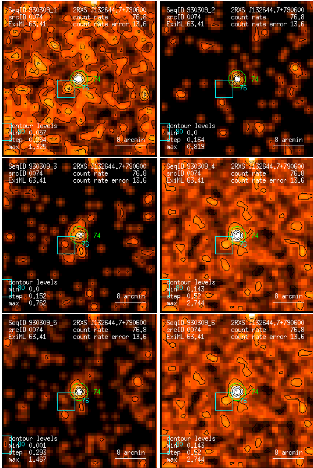
Figure 74: RASS 930309: detection 0074: band rate images, Gaussian filter: (1) PSPC channels 11 – 41, (2) 52 – 90, (3) 91 – 201, (4) 11 – 235, (5) 52 – 201, (6) 11 – 201. Broad band rates in counts/ks. Band rate contour levels in counts/ks/arcmin 2 .
