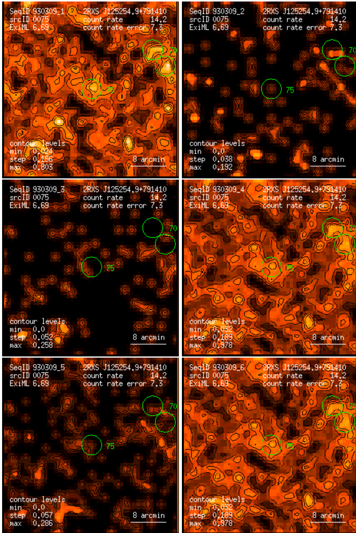
Figure 75: RASS 930309: detection 0075: band rate images, Gaussian filter: (1) PSPC channels 11 – 41, (2) 52 – 90, (3) 91 – 201, (4) 11 – 235, (5) 52 – 201, (6) 11 – 201. Broad band rates in counts/ks. Band rate contour levels in counts/ks/arcmin 2 .
