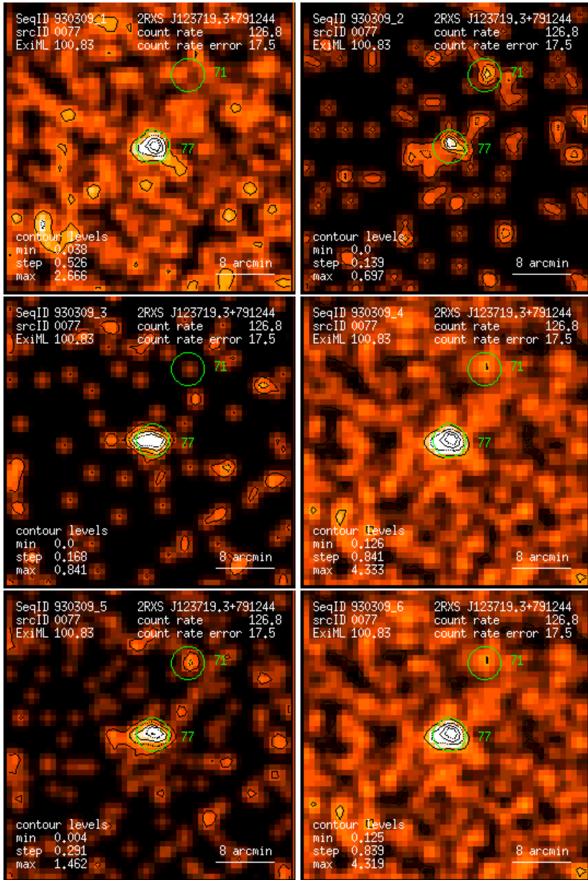
Figure 77: RASS 930309: detection 0077: band rate images, Gaussian filter: (1) PSPC channels 11 – 41, (2) 52 – 90, (3) 91 – 201, (4) 11 – 235, (5) 52 – 201, (6) 11 – 201. Broad band rates in counts/ks. Band rate contour levels in counts/ks/arcmin 2 .
