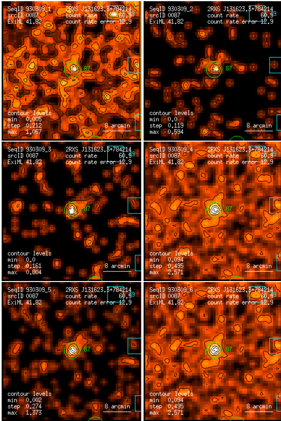
Figure 87: RASS 930309: detection 0087: band rate images, Gaussian filter: (1) PSPC channels 11 – 41, (2) 52 – 90, (3) 91 – 201, (4) 11 – 235, (5) 52 – 201, (6) 11 – 201. Broad band rates in counts/ks. Band rate contour levels in counts/ks/arcmin 2 .
