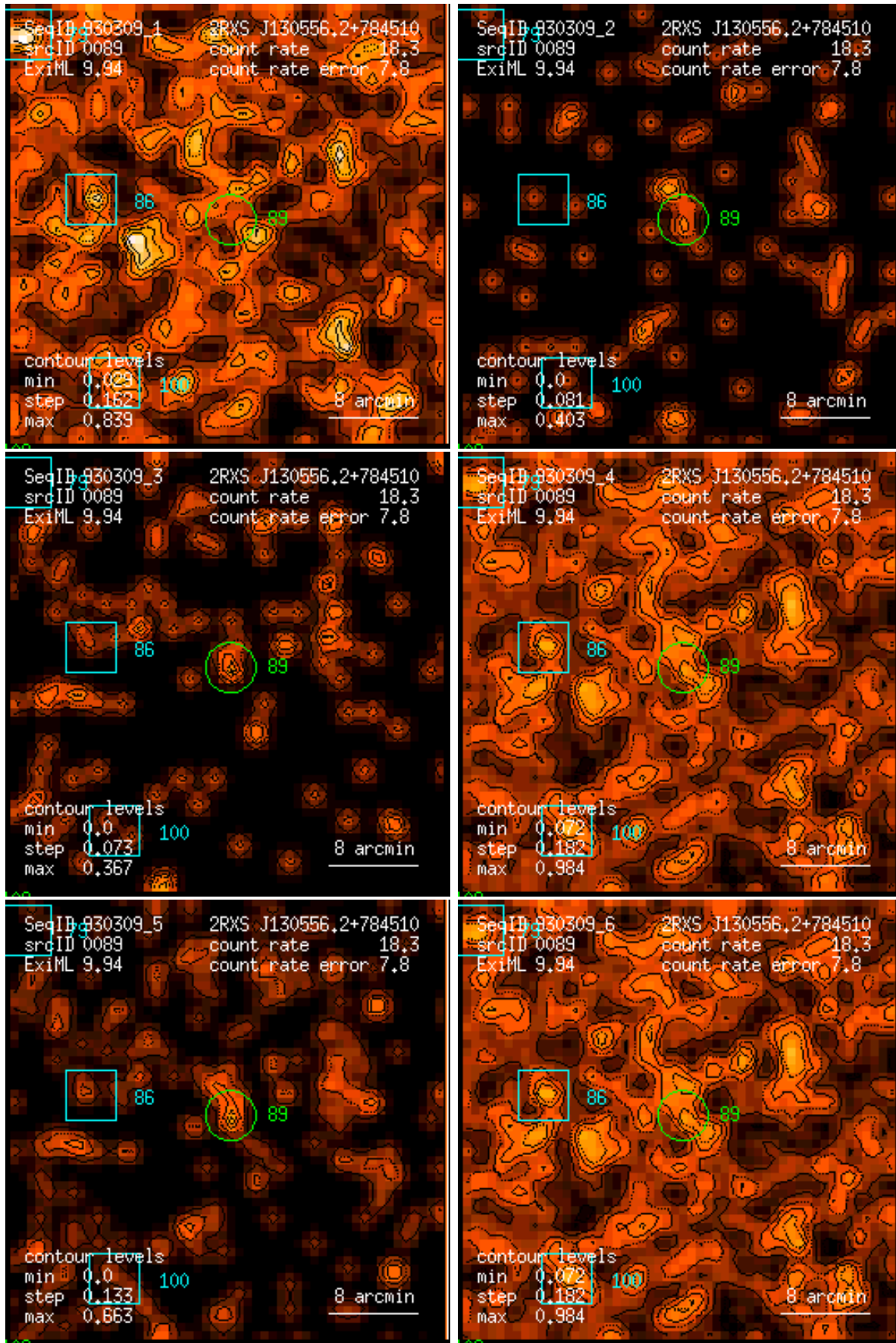
Figure 89: RASS 930309: detection 0089: band rate images, Gaussian filter: (1) PSPC channels 11 – 41, (2) 52 – 90, (3) 91 – 201, (4) 11 – 235, (5) 52 – 201, (6) 11 – 201. Broad band rates in counts/ks. Band rate contour levels in counts/ks/arcmin 2 .
