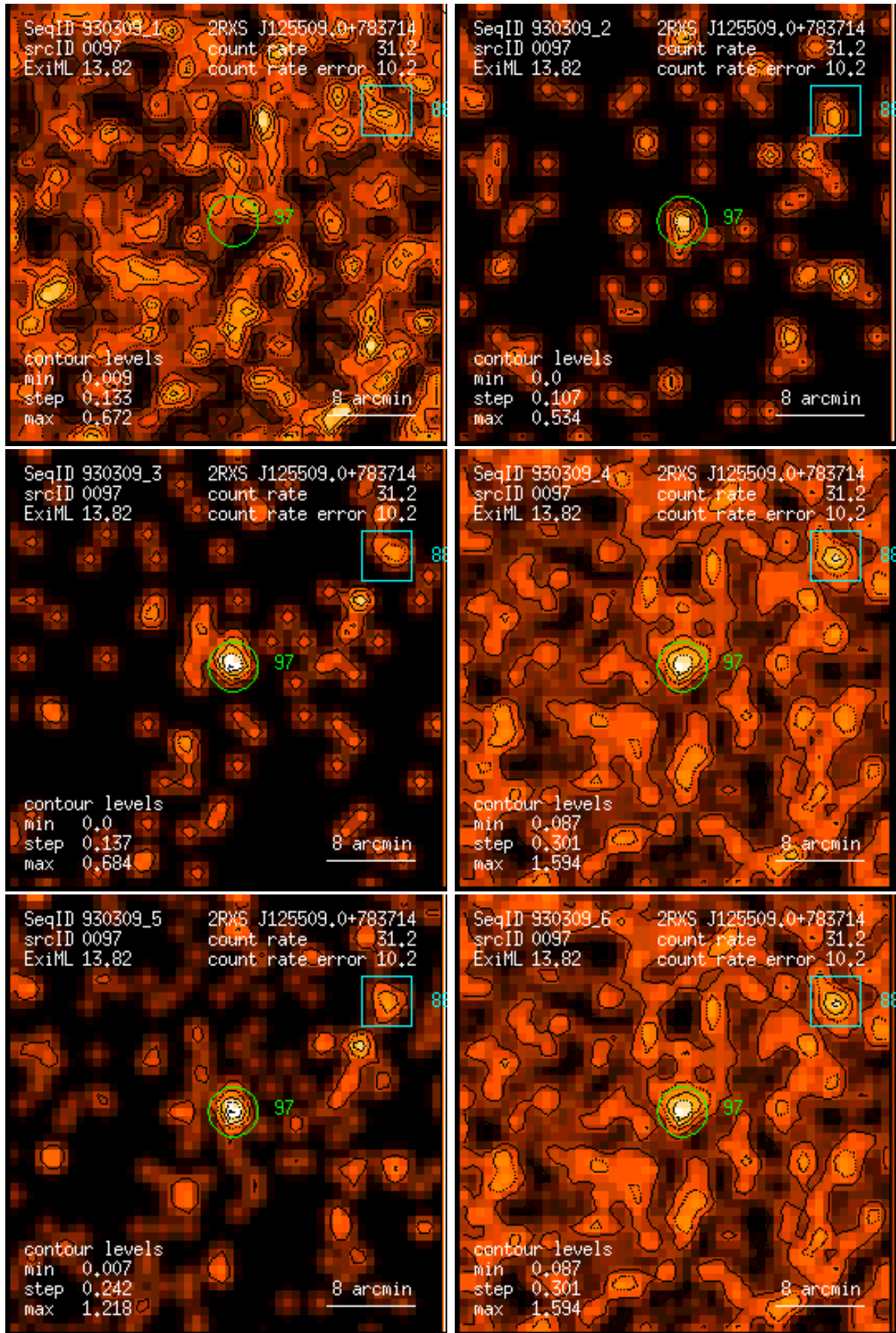
Figure 97: RASS 930309: detection 0097: band rate images, Gaussian filter: (1) PSPC channels 11 – 41, (2) 52 – 90, (3) 91 – 201, (4) 11 – 235, (5) 52 – 201, (6) 11 – 201. Broad band rates in counts/ks. Band rate contour levels in counts/ks/arcmin 2 .
