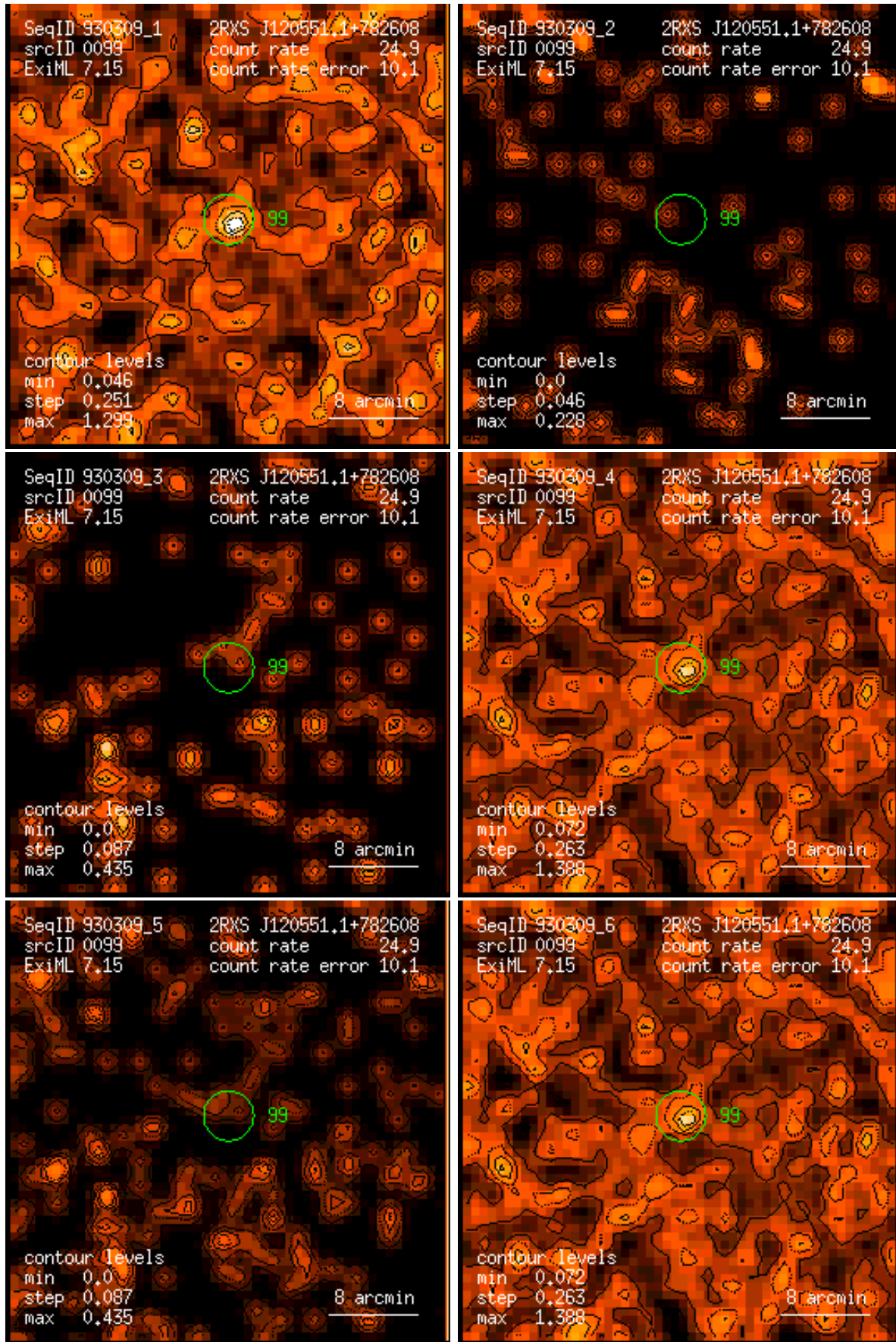
Figure 99: RASS 930309: detection 0099: band rate images, Gaussian filter: (1) PSPC channels 11 – 41, (2) 52 – 90, (3) 91 – 201, (4) 11 – 235, (5) 52 – 201, (6) 11 – 201. Broad band rates in counts/ks. Band rate contour levels in counts/ks/arcmin 2 .
