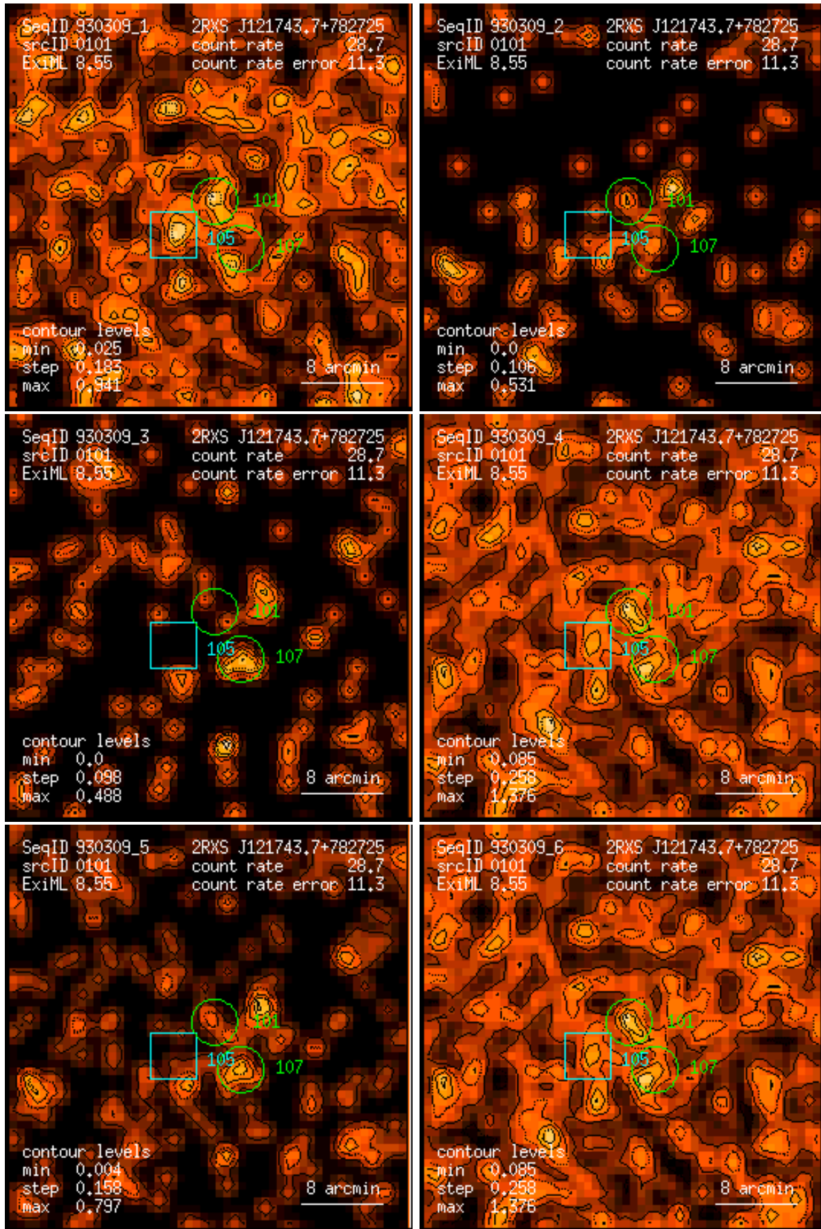
Figure 101: RASS 930309: detection 0101: band rate images, Gaussian filter: (1) PSPC channels 11 – 41, (2) 52 – 90, (3) 91 – 201, (4) 11 – 235, (5) 52 – 201, (6) 11 – 201. Broad band rates in counts/ks. Band rate contour levels in counts/ks/arcmin 2 .
