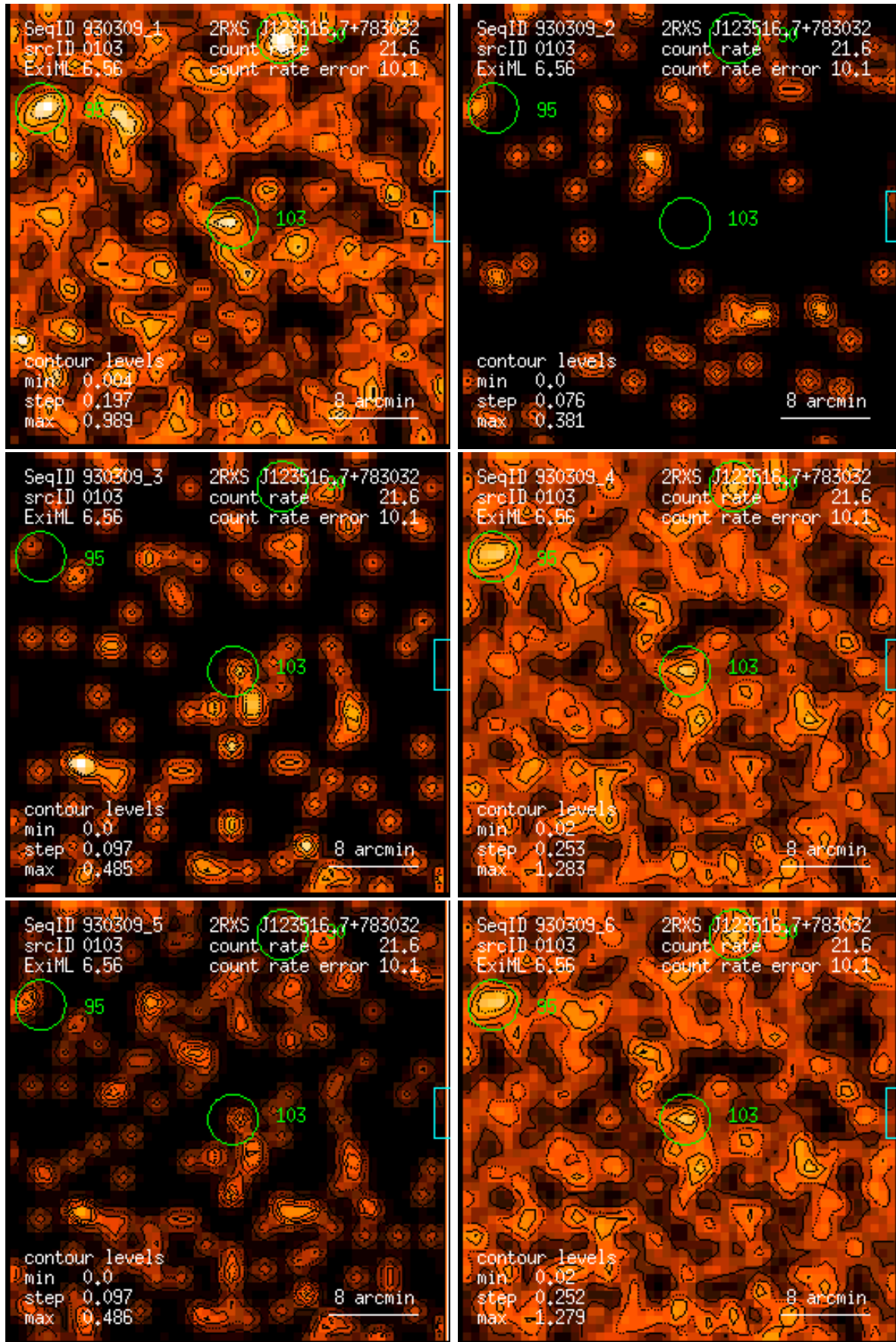
Figure 103: RASS 930309: detection 0103: band rate images, Gaussian filter: (1) PSPC channels 11 – 41, (2) 52 – 90, (3) 91 – 201, (4) 11 – 235, (5) 52 – 201, (6) 11 – 201. Broad band rates in counts/ks. Band rate contour levels in counts/ks/arcmin 2 .
