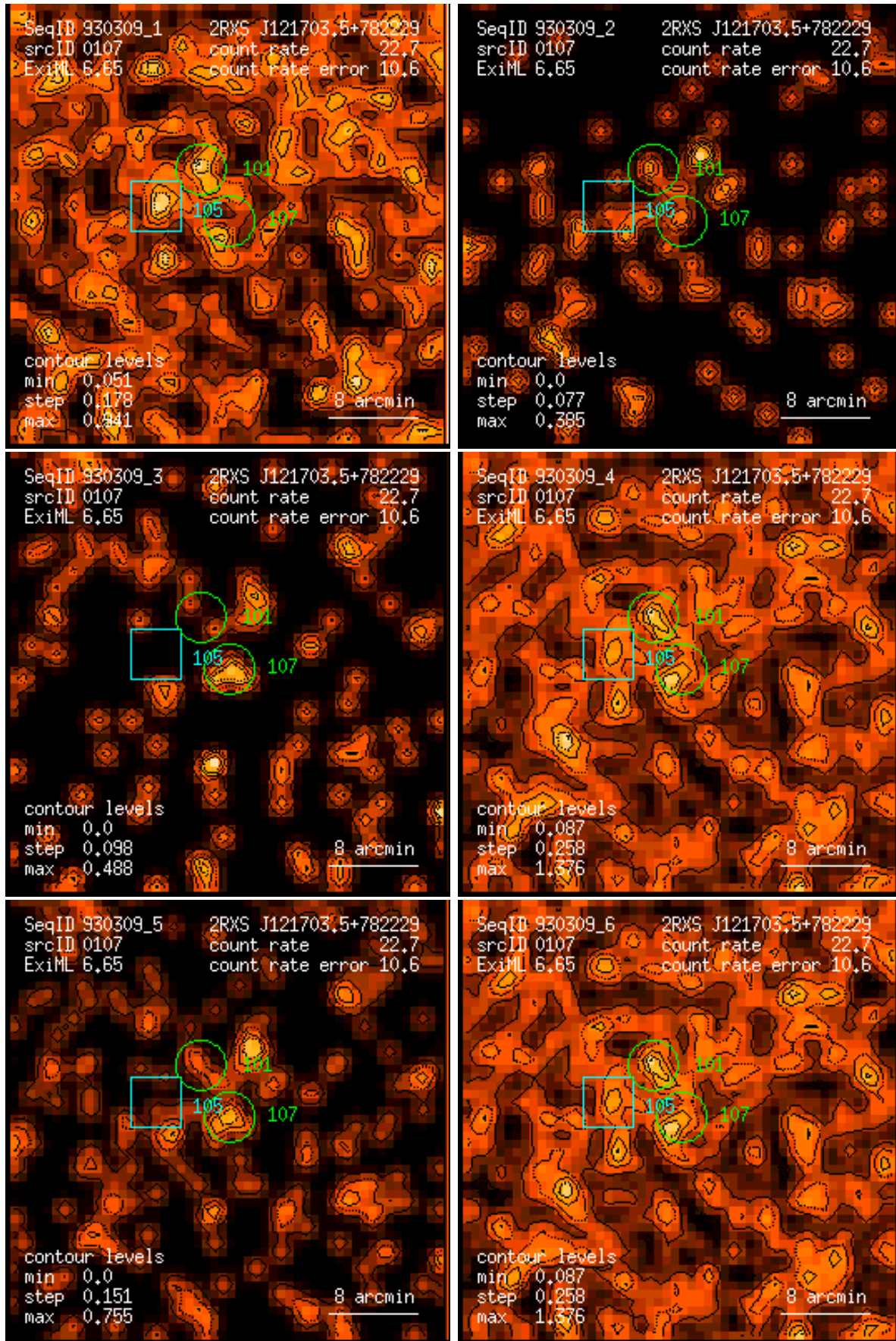
Figure 107: RASS 930309: detection 0107: band rate images, Gaussian filter: (1) PSPC channels 11 – 41, (2) 52 – 90, (3) 91 – 201, (4) 11 – 235, (5) 52 – 201, (6) 11 – 201. Broad band rates in counts/ks. Band rate contour levels in counts/ks/arcmin 2 .
