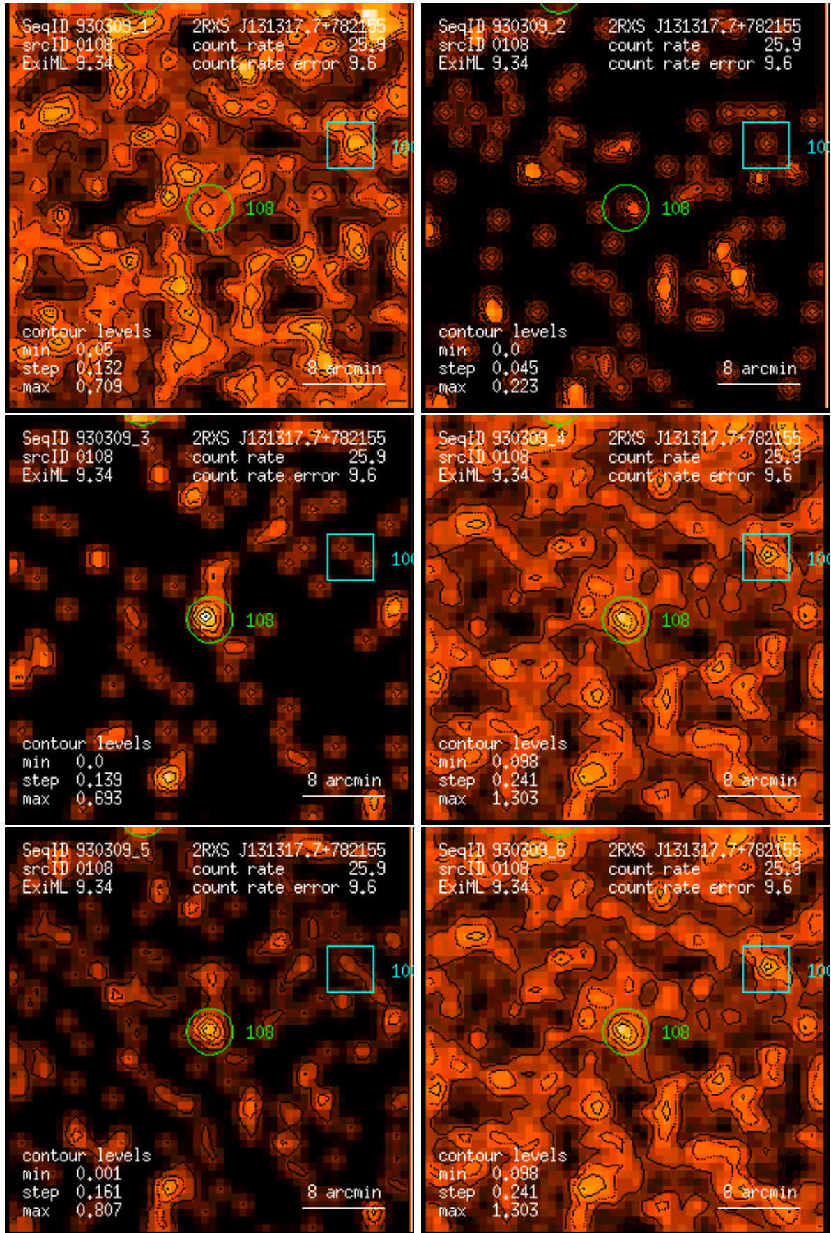
Figure 108: RASS 930309: detection 0108: band rate images, Gaussian filter: (1) PSPC channels 11 – 41, (2) 52 – 90, (3) 91 – 201, (4) 11 – 235, (5) 52 – 201, (6) 11 – 201. Broad band rates in counts/ks. Band rate contour levels in counts/ks/arcmin 2 .
