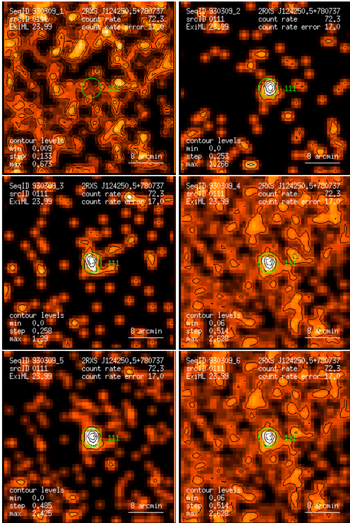
Figure 111: RASS 930309: detection 0111: band rate images, Gaussian filter: (1) PSPC channels 11 – 41, (2) 52 – 90, (3) 91 – 201, (4) 11 – 235, (5) 52 – 201, (6) 11 – 201. Broad band rates in counts/ks. Band rate contour levels in counts/ks/arcmin 2 .
