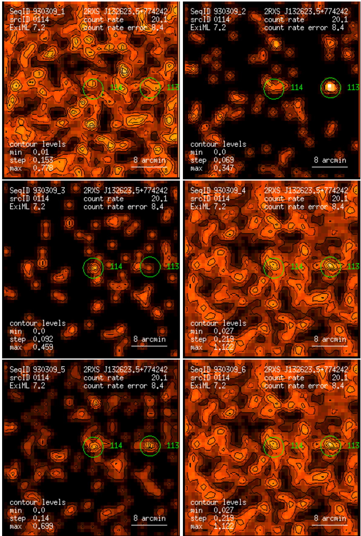
Figure 114: RASS 930309: detection 0114: band rate images, Gaussian filter: (1) PSPC channels 11 – 41, (2) 52 – 90, (3) 91 – 201, (4) 11 – 235, (5) 52 – 201, (6) 11 – 201. Broad band rates in counts/ks. Band rate contour levels in counts/ks/arcmin 2 .
