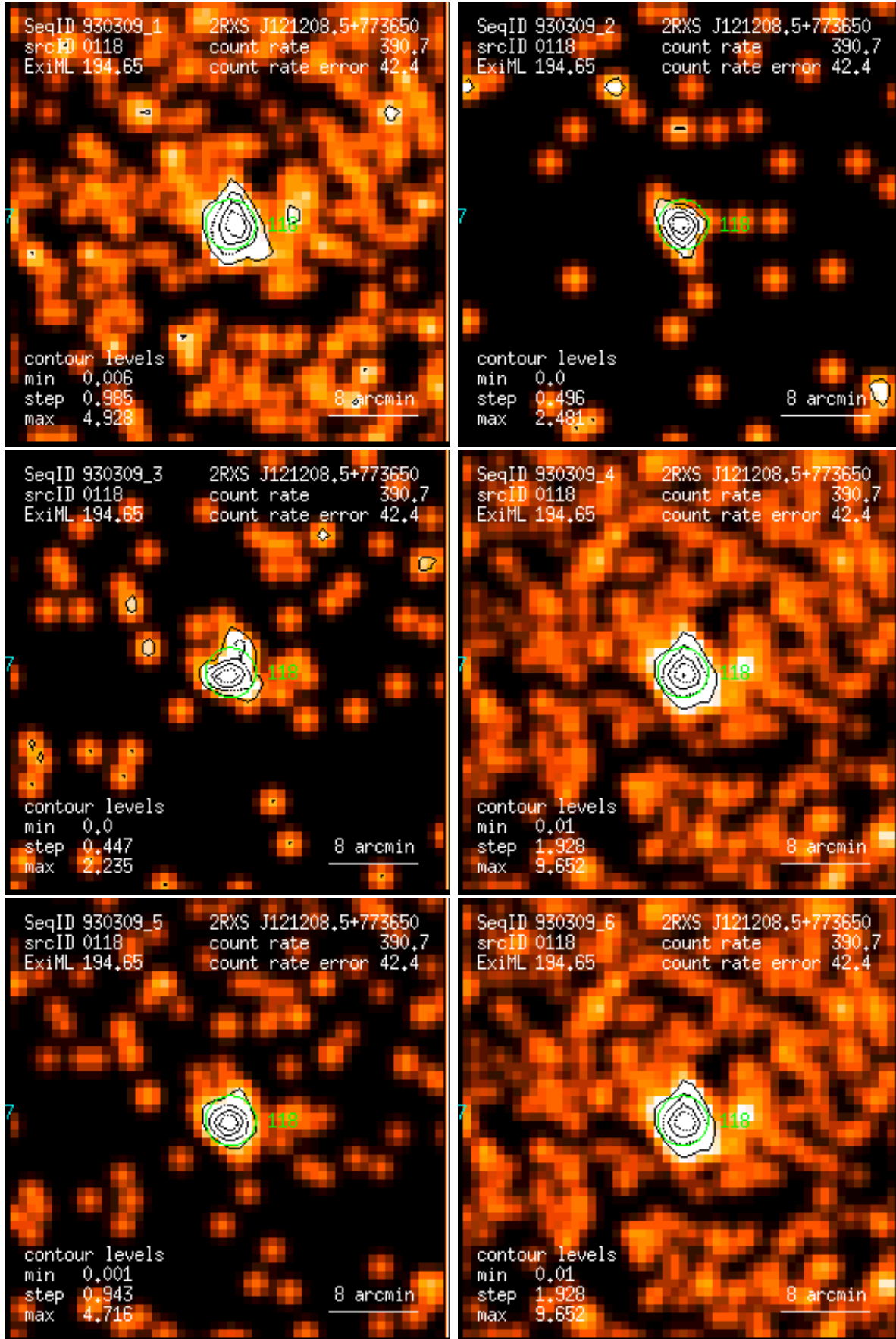
Figure 118: RASS 930309: detection 0118: band rate images, Gaussian filter: (1) PSPC channels 11 – 41, (2) 52 – 90, (3) 91 – 201, (4) 11 – 235, (5) 52 – 201, (6) 11 – 201. Broad band rates in counts/ks. Band rate contour levels in counts/ks/arcmin 2 .
