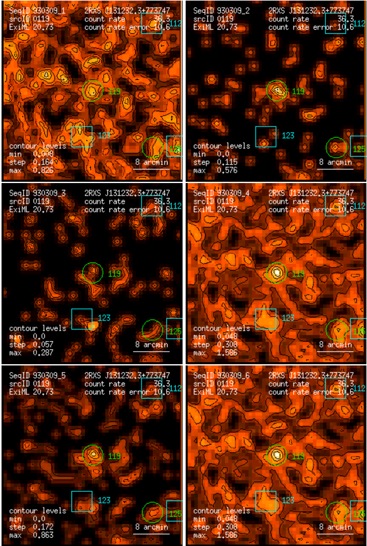
Figure 119: RASS 930309: detection 0119: band rate images, Gaussian filter: (1) PSPC channels 11 – 41, (2) 52 – 90, (3) 91 – 201, (4) 11 – 235, (5) 52 – 201, (6) 11 – 201. Broad band rates in counts/ks. Band rate contour levels in counts/ks/arcmin 2 .
