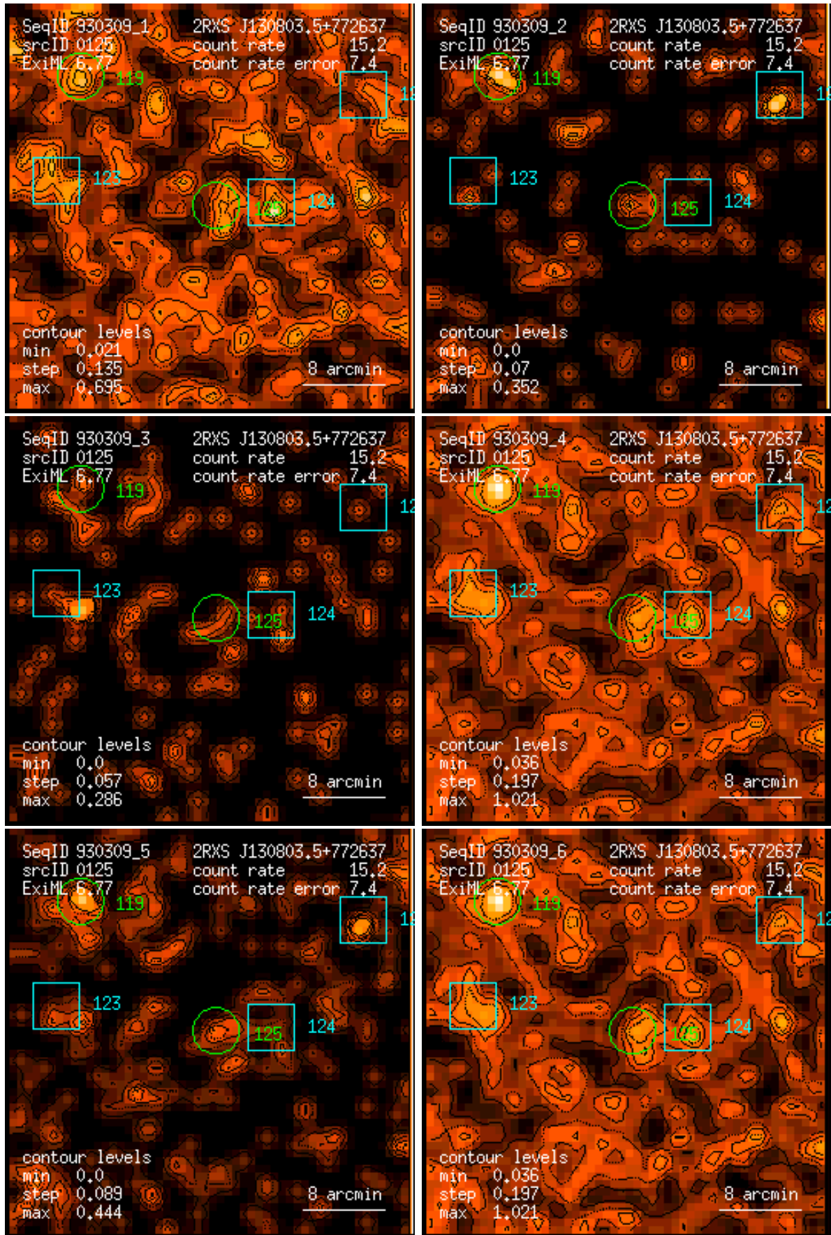
Figure 125: RASS 930309: detection 0125: band rate images, Gaussian filter: (1) PSPC channels 11 – 41, (2) 52 – 90, (3) 91 – 201, (4) 11 – 235, (5) 52 – 201, (6) 11 – 201. Broad band rates in counts/ks. Band rate contour levels in counts/ks/arcmin 2 .
