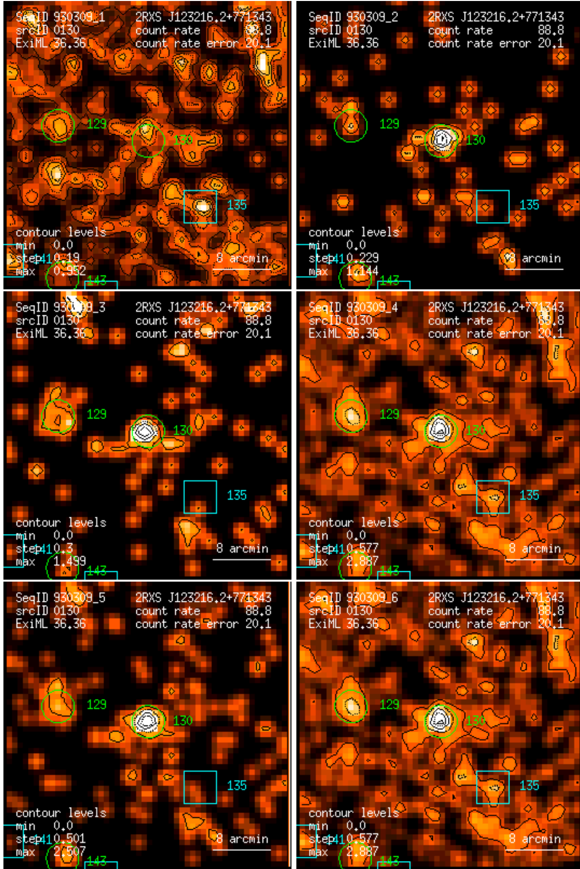
Figure 130: RASS 930309: detection 0130: band rate images, Gaussian filter: (1) PSPC channels 11 – 41, (2) 52 – 90, (3) 91 – 201, (4) 11 – 235, (5) 52 – 201, (6) 11 – 201. Broad band rates in counts/ks. Band rate contour levels in counts/ks/arcmin 2 .
