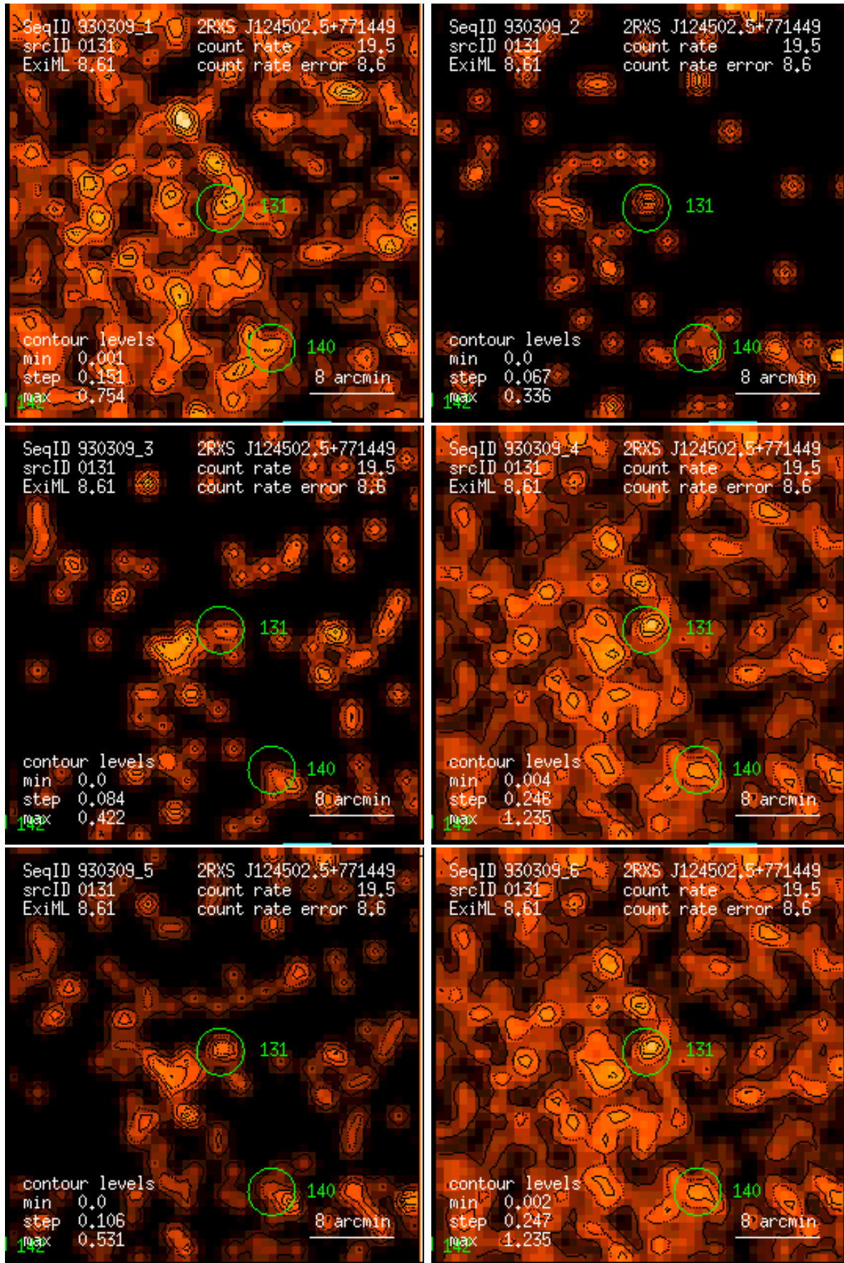
Figure 131: RASS 930309: detection 0131: band rate images, Gaussian filter: (1) PSPC channels 11 – 41, (2) 52 – 90, (3) 91 – 201, (4) 11 – 235, (5) 52 – 201, (6) 11 – 201. Broad band rates in counts/ks. Band rate contour levels in counts/ks/arcmin 2 .
