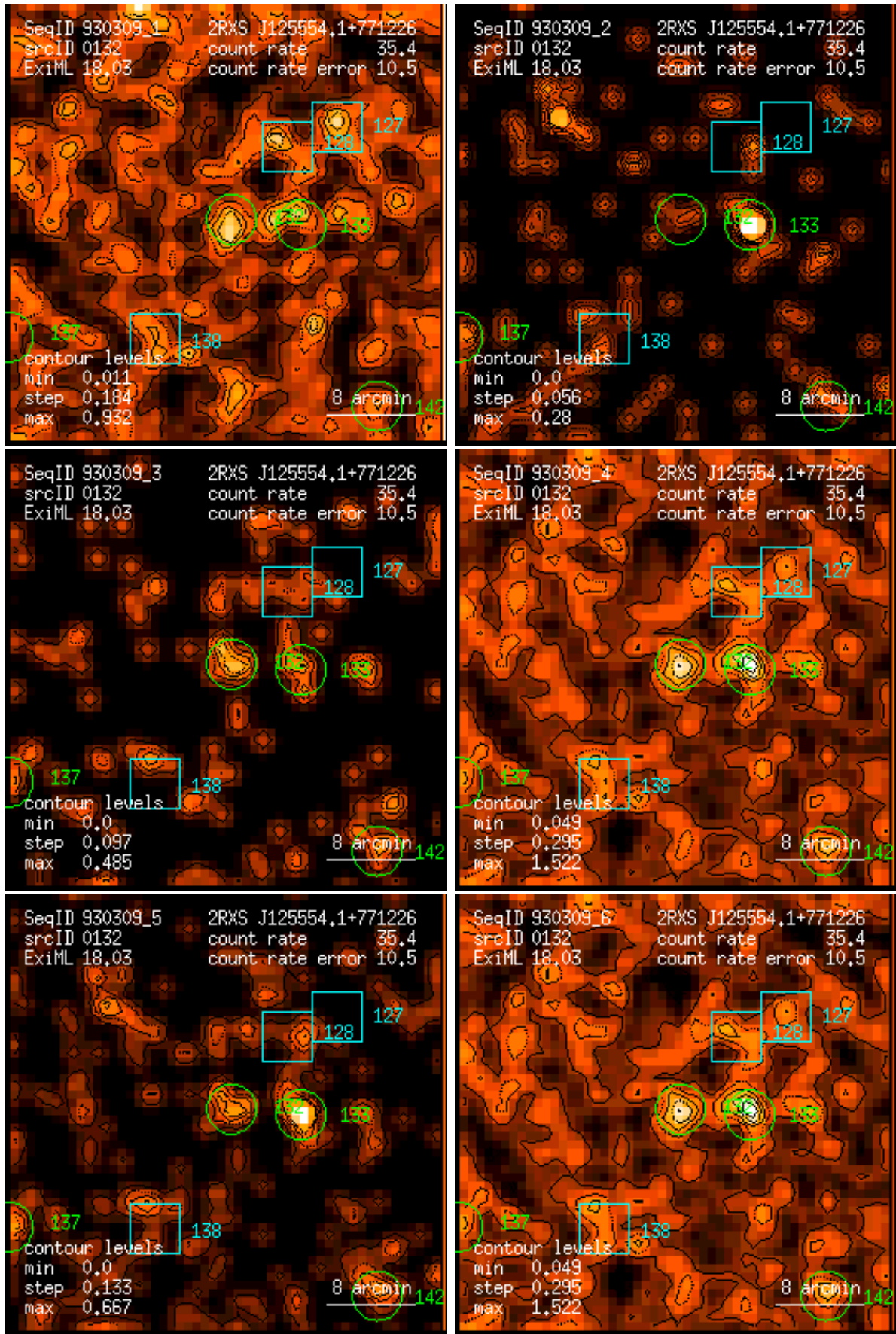
Figure 132: RASS 930309: detection 0132: band rate images, Gaussian filter: (1) PSPC channels 11 – 41, (2) 52 – 90, (3) 91 – 201, (4) 11 – 235, (5) 52 – 201, (6) 11 – 201. Broad band rates in counts/ks. Band rate contour levels in counts/ks/arcmin 2 .
