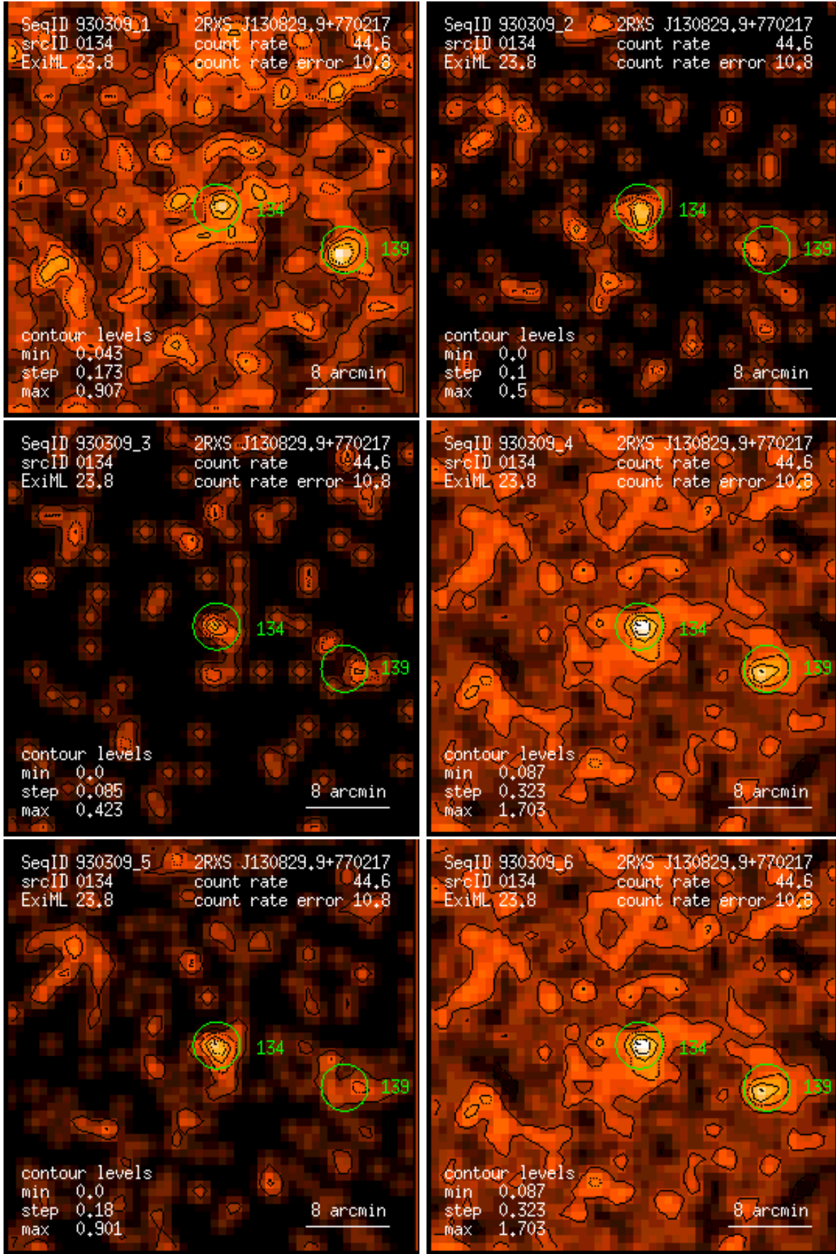
Figure 134: RASS 930309: detection 0134: band rate images, Gaussian filter: (1) PSPC channels 11 – 41, (2) 52 – 90, (3) 91 – 201, (4) 11 – 235, (5) 52 – 201, (6) 11 – 201. Broad band rates in counts/ks. Band rate contour levels in counts/ks/arcmin 2 .
