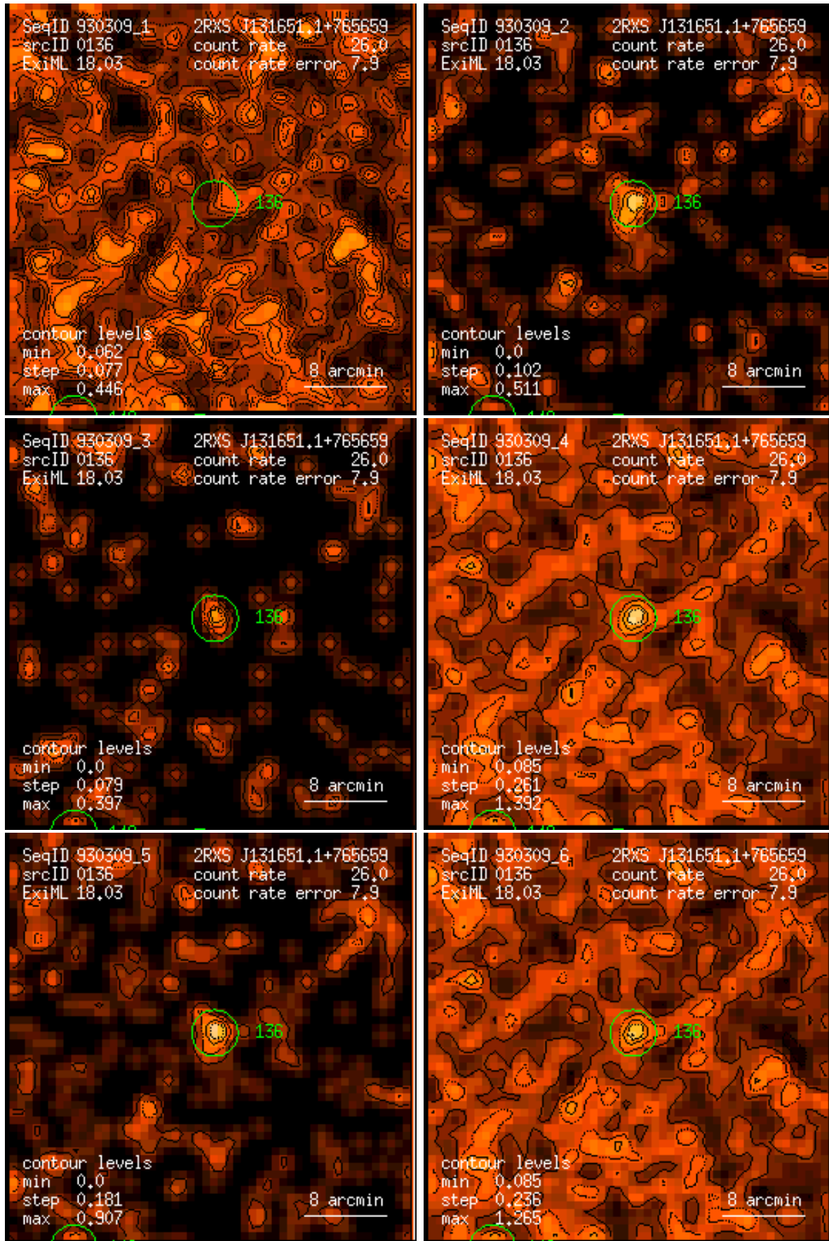
Figure 136: RASS 930309: detection 0136: band rate images, Gaussian filter: (1) PSPC channels 11 – 41, (2) 52 – 90, (3) 91 – 201, (4) 11 – 235, (5) 52 – 201, (6) 11 – 201. Broad band rates in counts/ks. Band rate contour levels in counts/ks/arcmin 2 .
