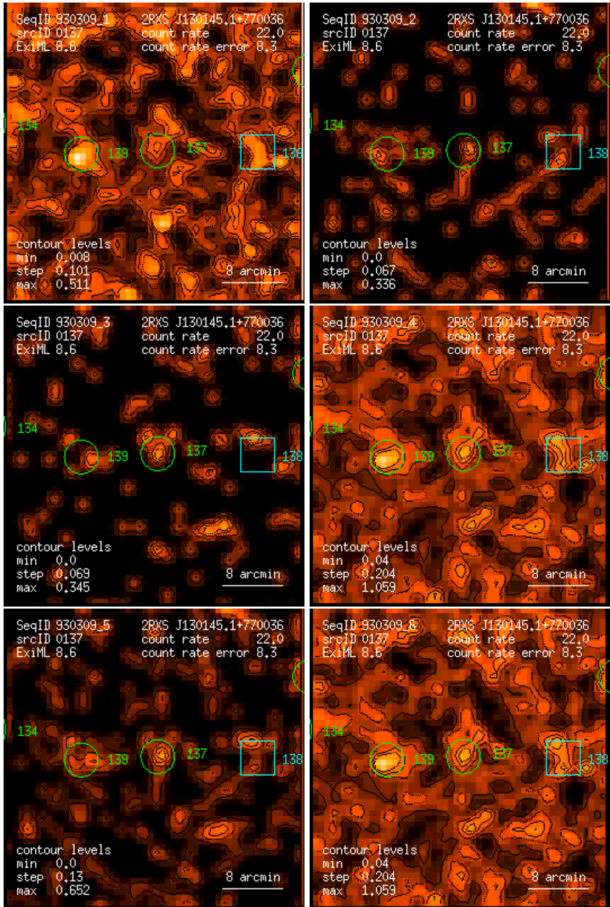
Figure 137: RASS 930309: detection 0137: band rate images, Gaussian filter: (1) PSPC channels 11 – 41, (2) 52 – 90, (3) 91 – 201, (4) 11 – 235, (5) 52 – 201, (6) 11 – 201. Broad band rates in counts/ks. Band rate contour levels in counts/ks/arcmin 2 .
