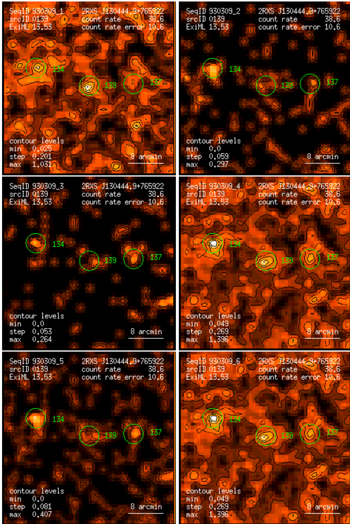
Figure 139: RASS 930309: detection 0139: band rate images, Gaussian filter: (1) PSPC channels 11 – 41, (2) 52 – 90, (3) 91 – 201, (4) 11 – 235, (5) 52 – 201, (6) 11 – 201. Broad band rates in counts/ks. Band rate contour levels in counts/ks/arcmin 2 .
