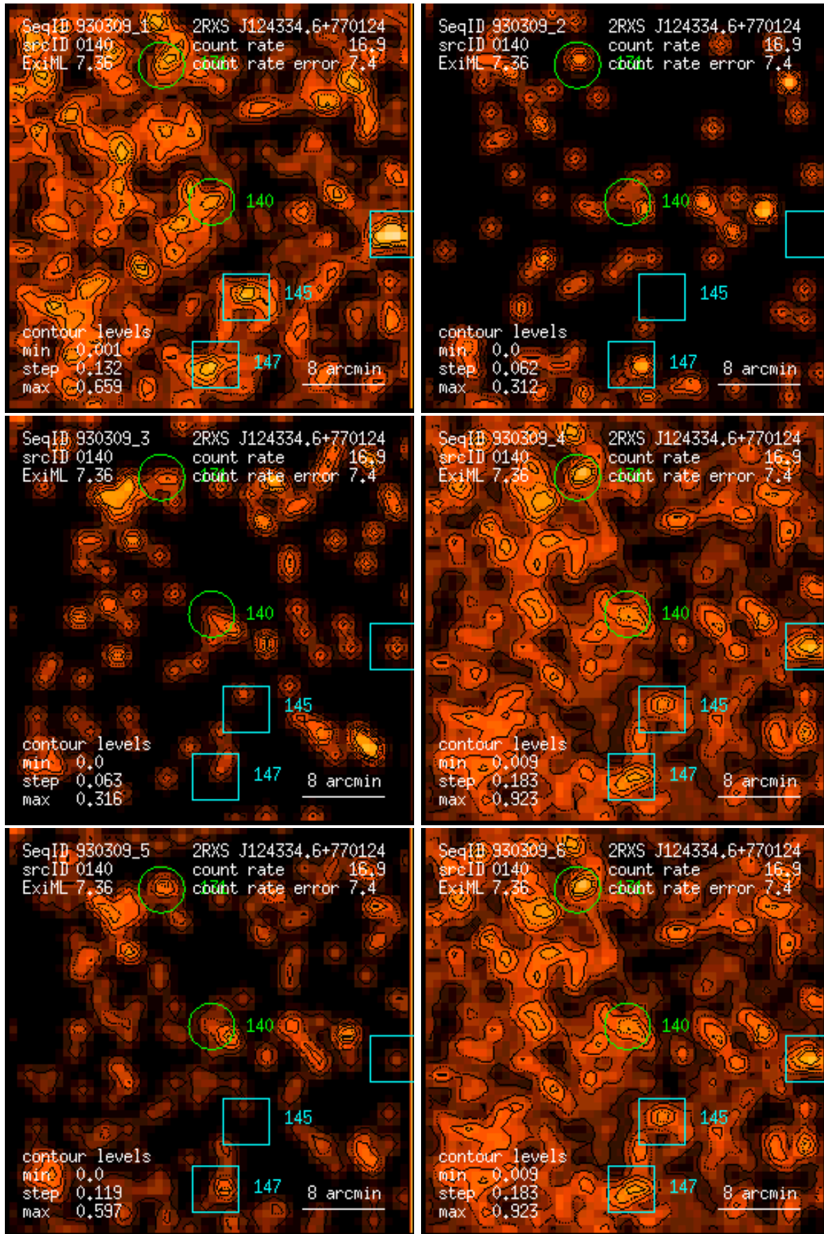
Figure 140: RASS 930309: detection 0140: band rate images, Gaussian filter: (1) PSPC channels 11 – 41, (2) 52 – 90, (3) 91 – 201, (4) 11 – 235, (5) 52 – 201, (6) 11 – 201. Broad band rates in counts/ks. Band rate contour levels in counts/ks/arcmin 2 .
