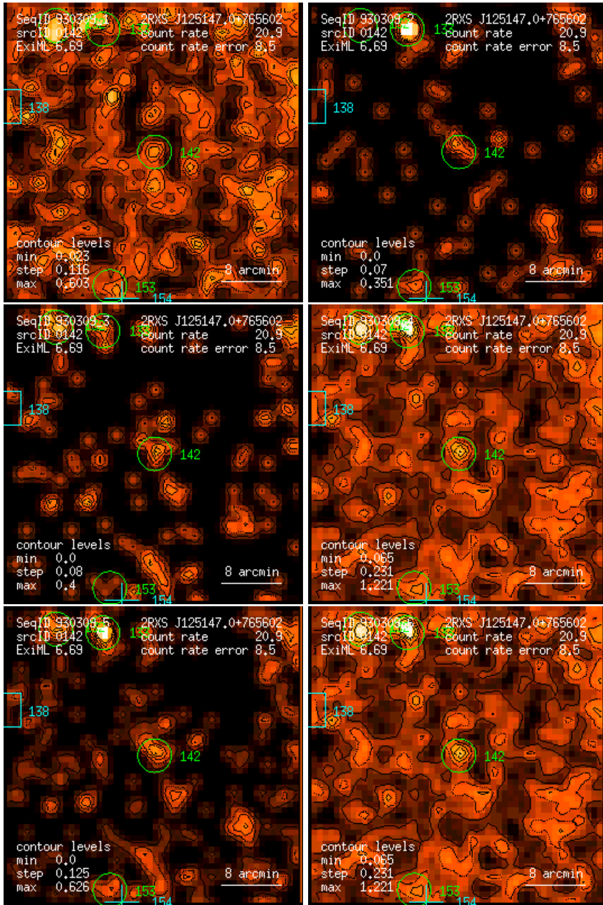
Figure 142: RASS 930309: detection 0142: band rate images, Gaussian filter: (1) PSPC channels 11 – 41, (2) 52 – 90, (3) 91 – 201, (4) 11 – 235, (5) 52 – 201, (6) 11 – 201. Broad band rates in counts/ks. Band rate contour levels in counts/ks/arcmin 2 .
