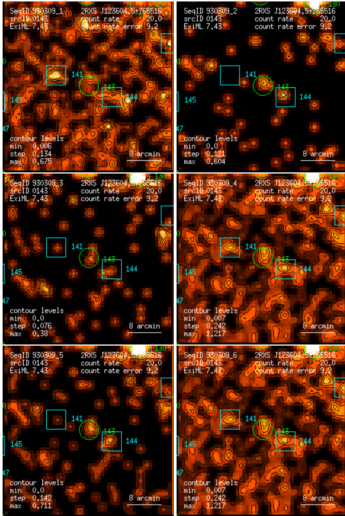
Figure 143: RASS 930309: detection 0143: band rate images, Gaussian filter: (1) PSPC channels 11 – 41, (2) 52 – 90, (3) 91 – 201, (4) 11 – 235, (5) 52 – 201, (6) 11 – 201. Broad band rates in counts/ks. Band rate contour levels in counts/ks/arcmin 2 .
