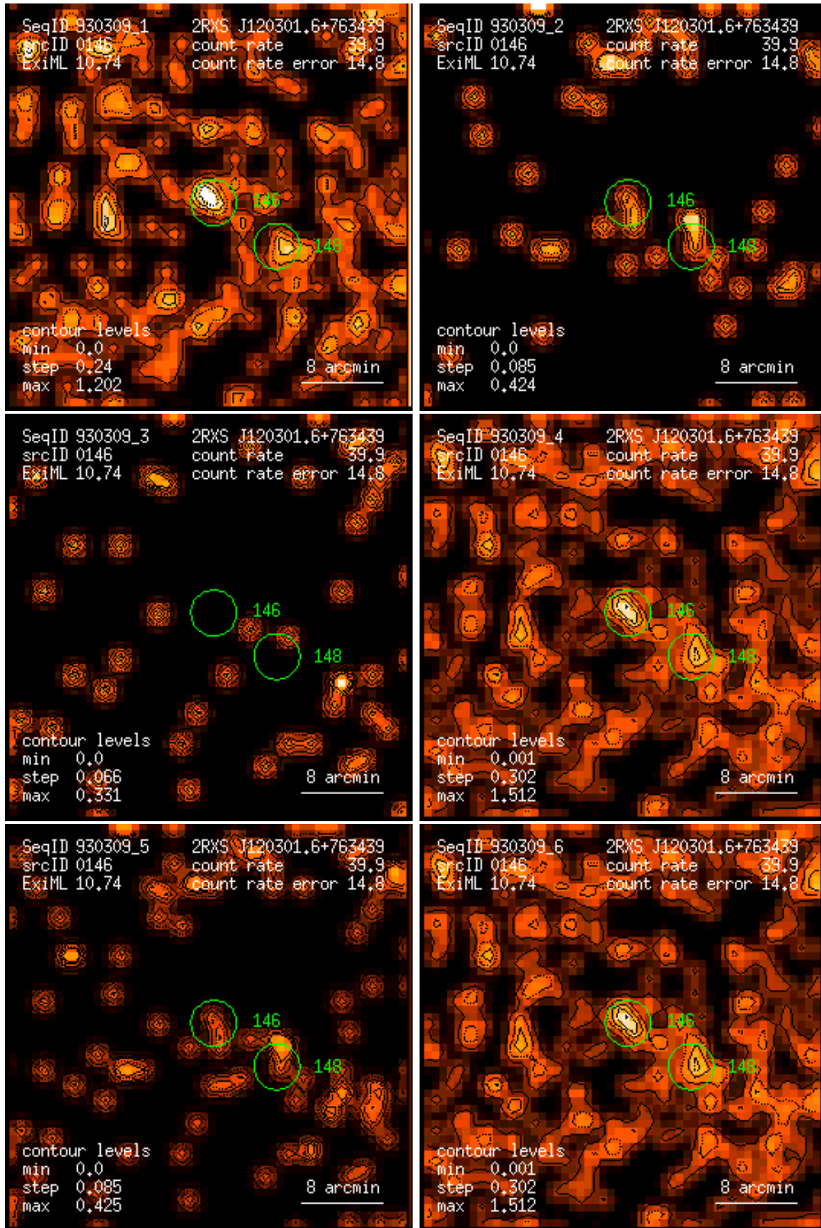
Figure 146: RASS 930309: detection 0146: band rate images, Gaussian filter: (1) PSPC channels 11 – 41, (2) 52 – 90, (3) 91 – 201, (4) 11 – 235, (5) 52 – 201, (6) 11 – 201. Broad band rates in counts/ks. Band rate contour levels in counts/ks/arcmin 2 .
