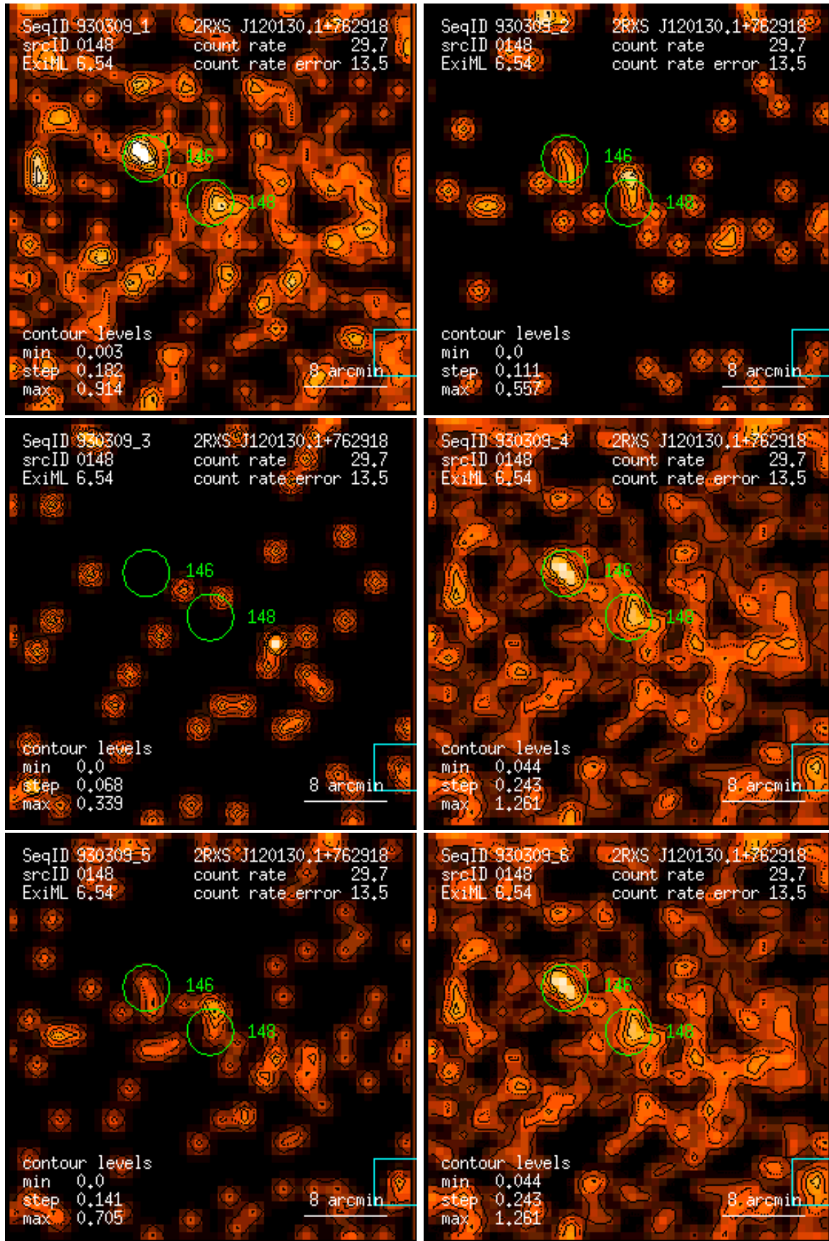
Figure 148: RASS 930309: detection 0148: band rate images, Gaussian filter: (1) PSPC channels 11 – 41, (2) 52 – 90, (3) 91 – 201, (4) 11 – 235, (5) 52 – 201, (6) 11 – 201. Broad band rates in counts/ks. Band rate contour levels in counts/ks/arcmin 2 .
