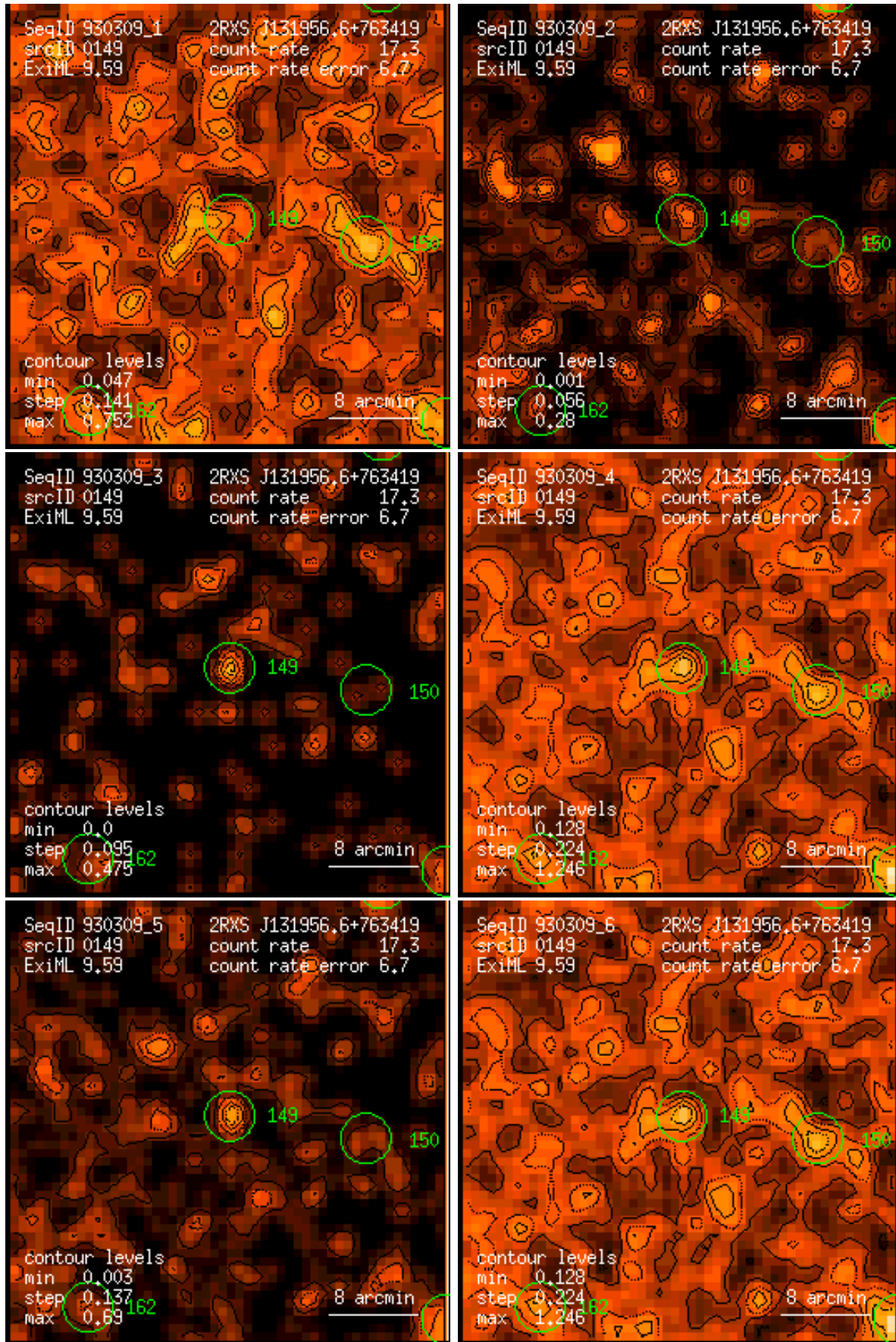
Figure 149: RASS 930309: detection 0149: band rate images, Gaussian filter: (1) PSPC channels 11 – 41, (2) 52 – 90, (3) 91 – 201, (4) 11 – 235, (5) 52 – 201, (6) 11 – 201. Broad band rates in counts/ks. Band rate contour levels in counts/ks/arcmin 2 .
