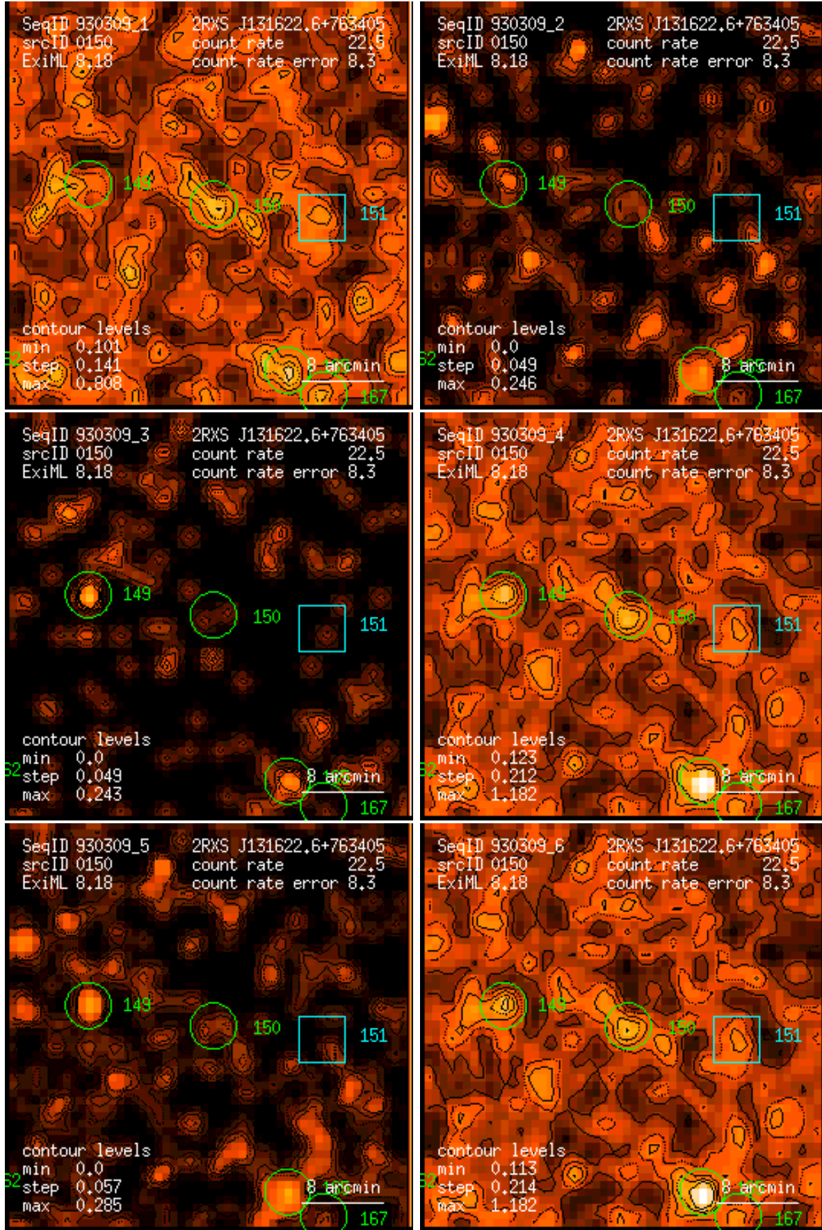
Figure 150: RASS 930309: detection 0150: band rate images, Gaussian filter: (1) PSPC channels 11 – 41, (2) 52 – 90, (3) 91 – 201, (4) 11 – 235, (5) 52 – 201, (6) 11 – 201. Broad band rates in counts/ks. Band rate contour levels in counts/ks/arcmin 2 .
