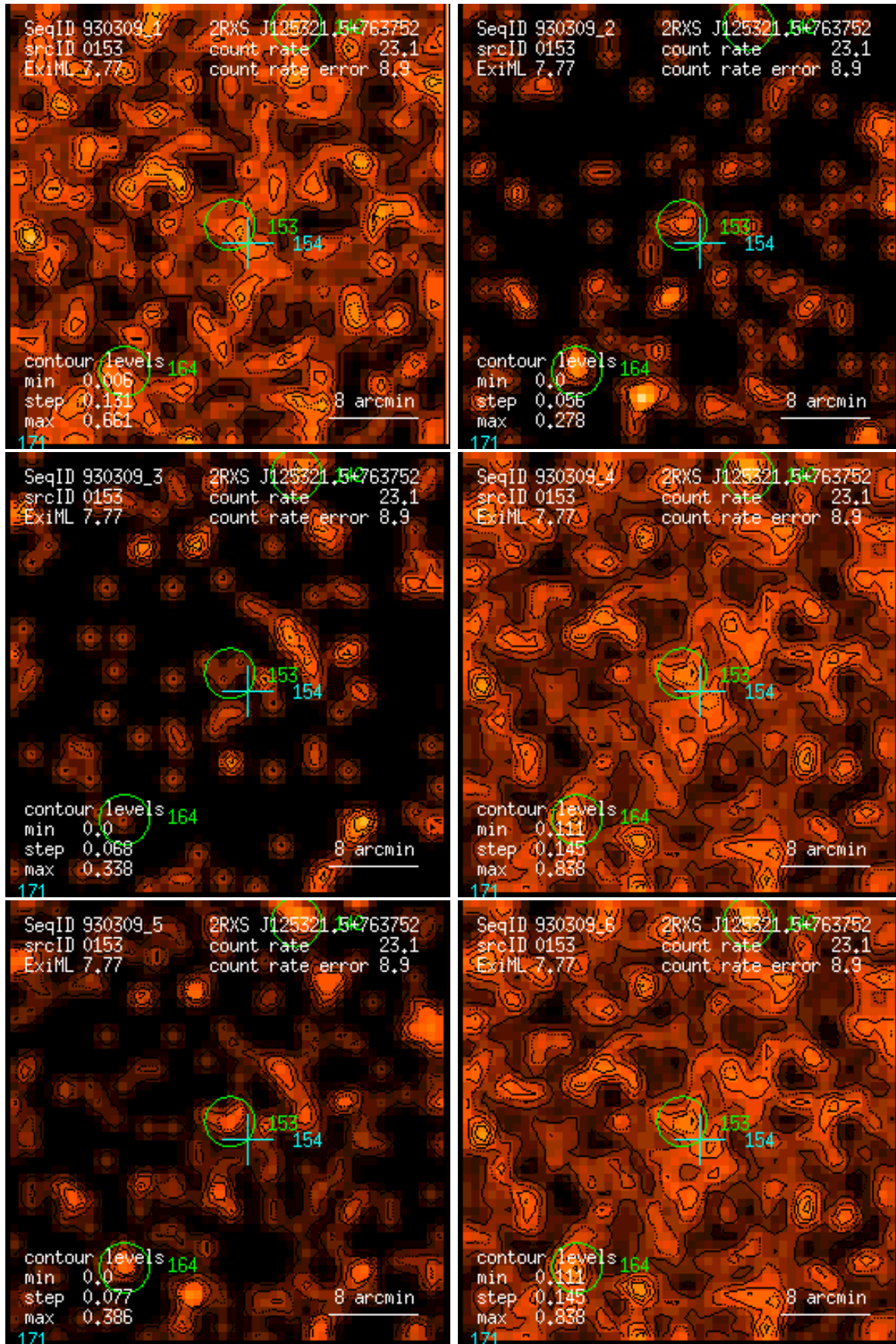
Figure 153: RASS 930309: detection 0153: band rate images, Gaussian filter: (1) PSPC channels 11 – 41, (2) 52 – 90, (3) 91 – 201, (4) 11 – 235, (5) 52 – 201, (6) 11 – 201. Broad band rates in counts/ks. Band rate contour levels in counts/ks/arcmin 2 .
