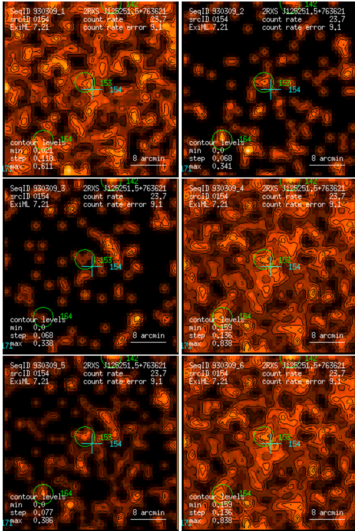
Figure 154: RASS 930309: detection 0154: band rate images, Gaussian filter: (1) PSPC channels 11 – 41, (2) 52 – 90, (3) 91 – 201, (4) 11 – 235, (5) 52 – 201, (6) 11 – 201. Broad band rates in counts/ks. Band rate contour levels in counts/ks/arcmin 2 .
