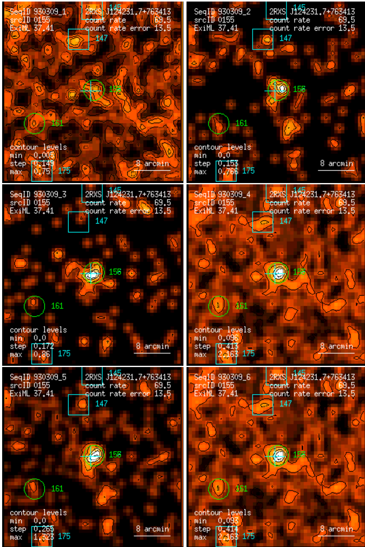
Figure 155: RASS 930309: detection 0155: band rate images, Gaussian filter: (1) PSPC channels 11 – 41, (2) 52 – 90, (3) 91 – 201, (4) 11 – 235, (5) 52 – 201, (6) 11 – 201. Broad band rates in counts/ks. Band rate contour levels in counts/ks/arcmin 2 .
