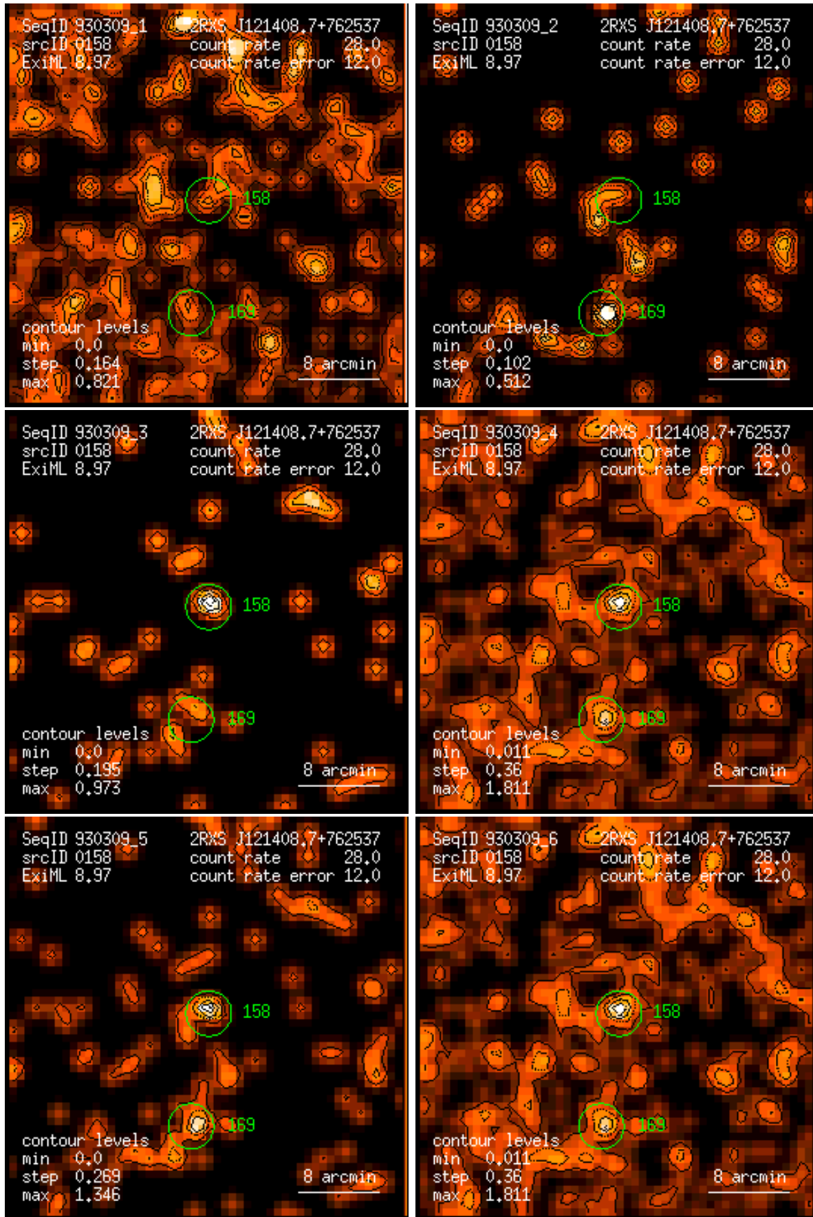
Figure 158: RASS 930309: detection 0158: band rate images, Gaussian filter: (1) PSPC channels 11 – 41, (2) 52 – 90, (3) 91 – 201, (4) 11 – 235, (5) 52 – 201, (6) 11 – 201. Broad band rates in counts/ks. Band rate contour levels in counts/ks/arcmin 2 .
