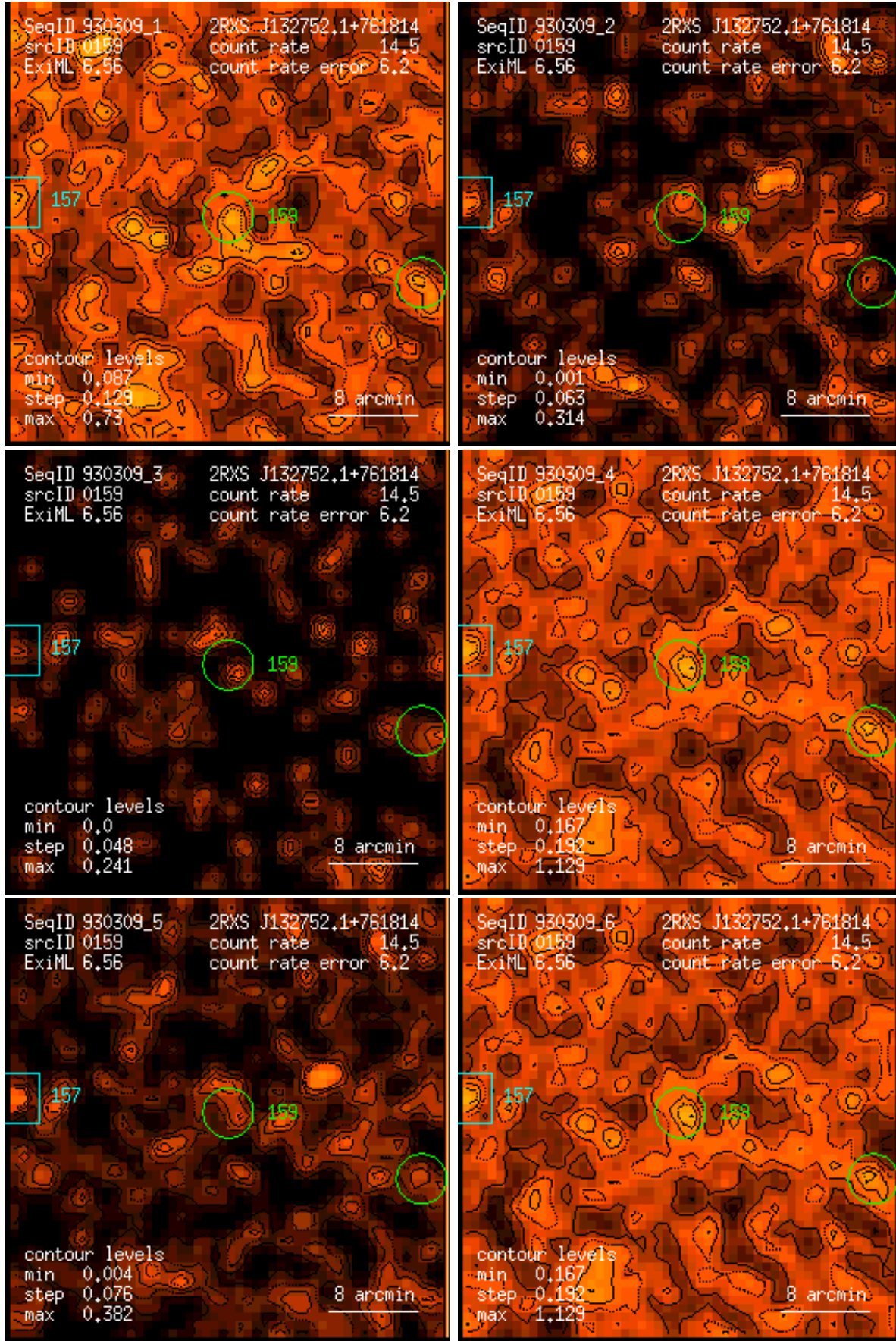
Figure 159: RASS 930309: detection 0159: band rate images, Gaussian filter: (1) PSPC channels 11 – 41, (2) 52 – 90, (3) 91 – 201, (4) 11 – 235, (5) 52 – 201, (6) 11 – 201. Broad band rates in counts/ks. Band rate contour levels in counts/ks/arcmin 2 .
