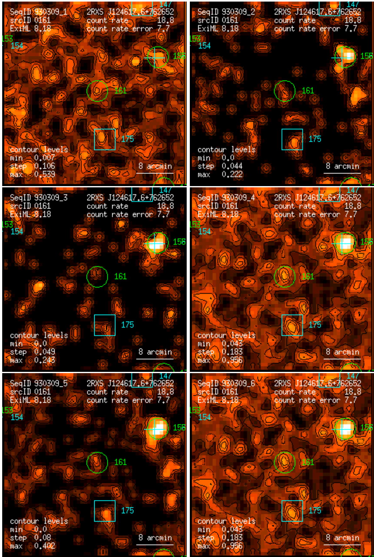
Figure 161: RASS 930309: detection 0161: band rate images, Gaussian filter: (1) PSPC channels 11 – 41, (2) 52 – 90, (3) 91 – 201, (4) 11 – 235, (5) 52 – 201, (6) 11 – 201. Broad band rates in counts/ks. Band rate contour levels in counts/ks/arcmin 2 .
