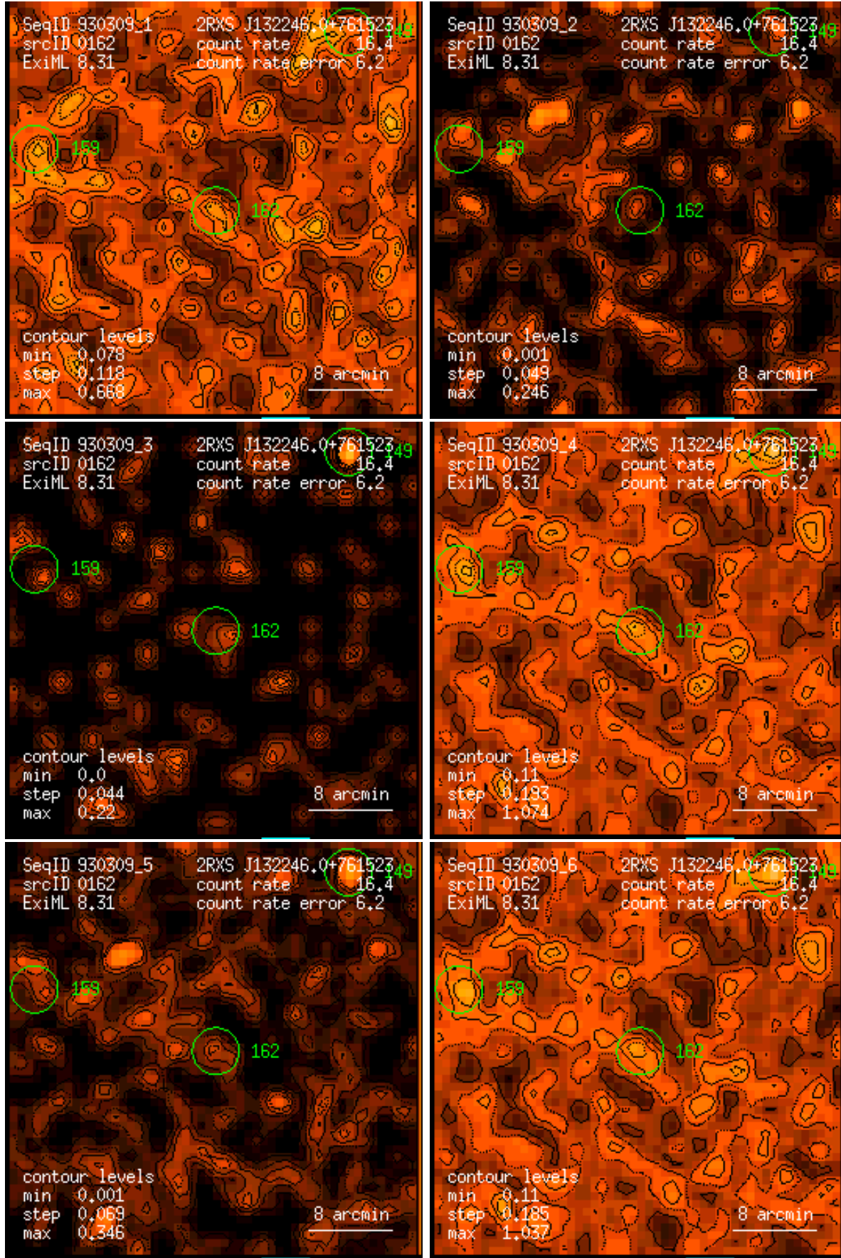
Figure 162: RASS 930309: detection 0162: band rate images, Gaussian filter: (1) PSPC channels 11 – 41, (2) 52 – 90, (3) 91 – 201, (4) 11 – 235, (5) 52 – 201, (6) 11 – 201. Broad band rates in counts/ks. Band rate contour levels in counts/ks/arcmin 2 .
