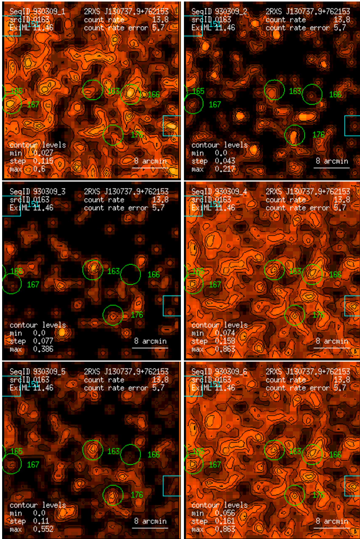
Figure 163: RASS 930309: detection 0163: band rate images, Gaussian filter: (1) PSPC channels 11 – 41, (2) 52 – 90, (3) 91 – 201, (4) 11 – 235, (5) 52 – 201, (6) 11 – 201. Broad band rates in counts/ks. Band rate contour levels in counts/ks/arcmin 2 .
